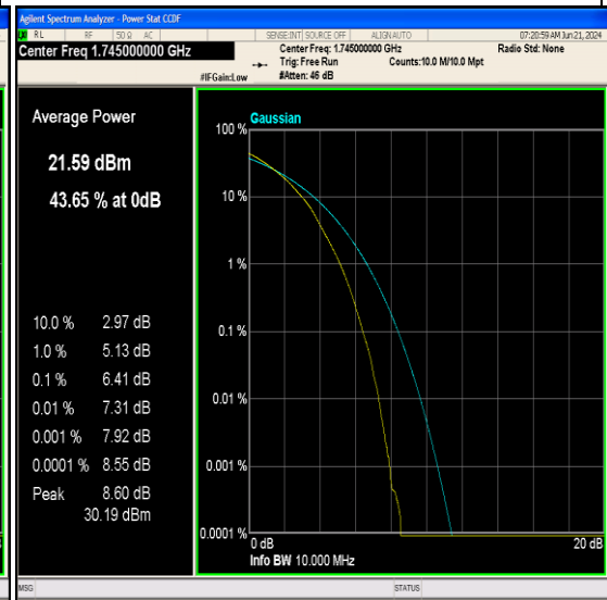
Band66-10MHz-64QAM-132322-50RB#0-PASS
