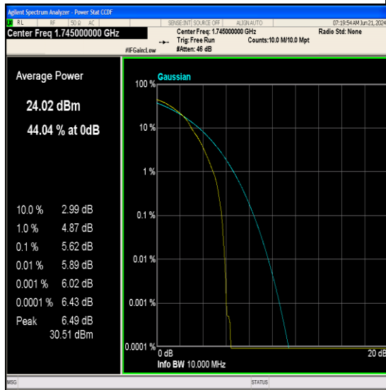
Band66-10MHz-64QAM-132322-1RB#0-PASS
