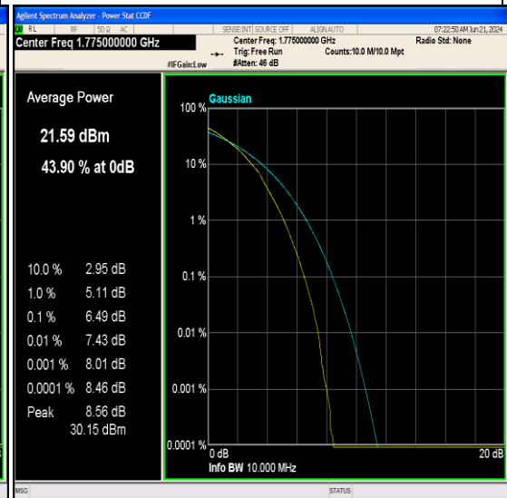
Band66-10MHz-64QAM-132622-50RB#0-PASS
