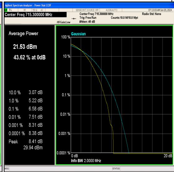
Band12-1.4MHz-64QAM-23173-6RB#0-PASS
