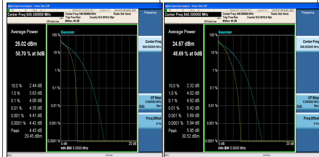
Band5-5MHz-QPSK-20625-1RB#0-PASS
