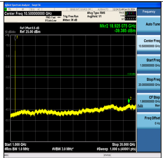
Band4-1413-1000~20000MHz-PASS
