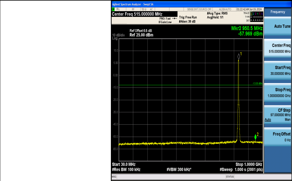
Band5-4182-1-30~1000MHz-PASS
