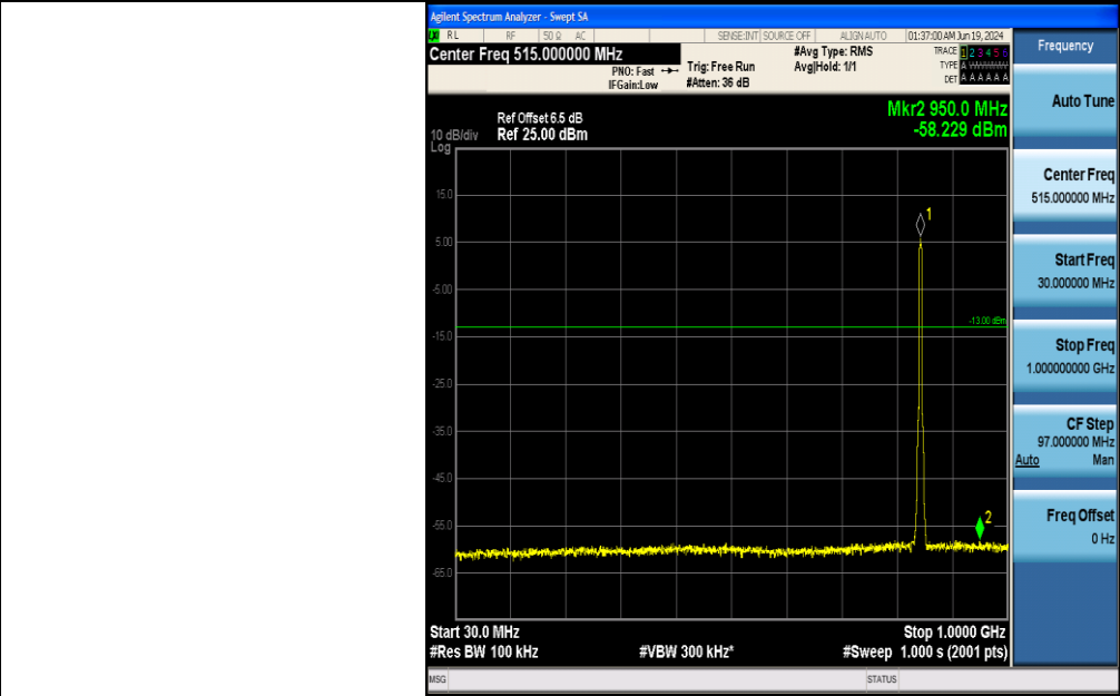
Band5-4233-1-30~1000MHz-PASS
