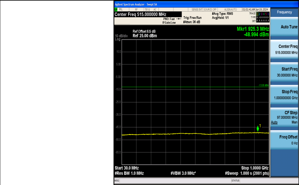
Band4-1413-1-30~1000MHz-PASS
