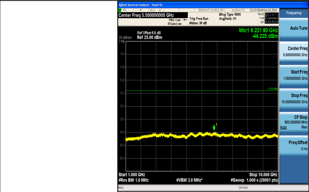
Band5-4233-1-1000~10000MHz-PASS
