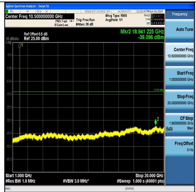
Band2-9538-1000~20000MHz-PASS
