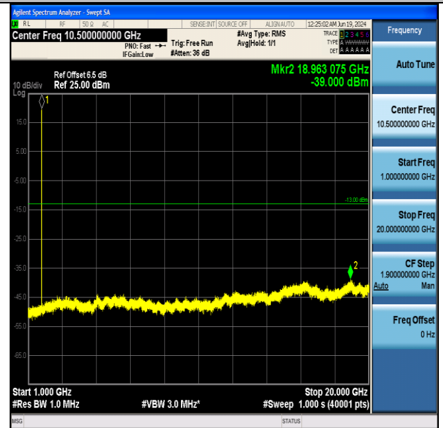
Band4-1513-1000~20000MHz-PASS
