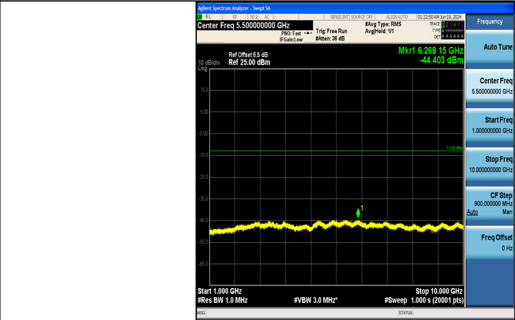
Band5-4182-1-1000~10000MHz-PASS
