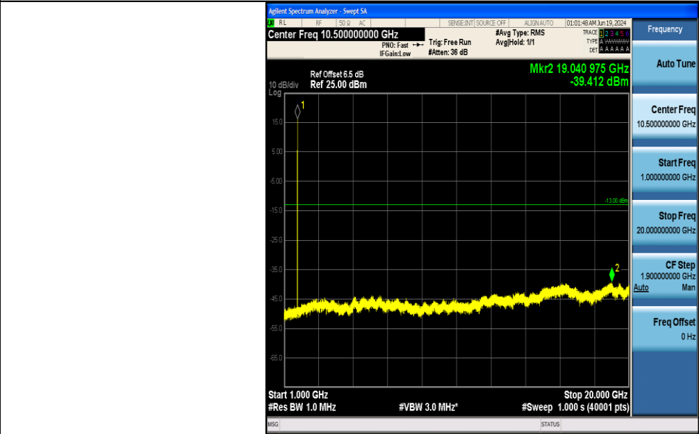
Band4-1413-1-1000~20000MHz-PASS
