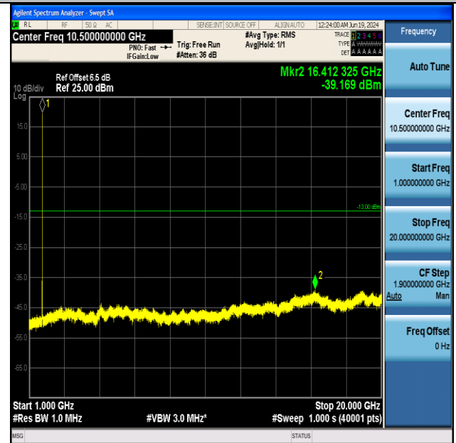
Band4-1312-1000~20000MHz-PASS
