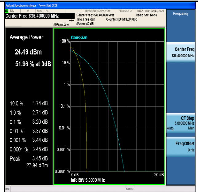
Band5-4182-PASS
