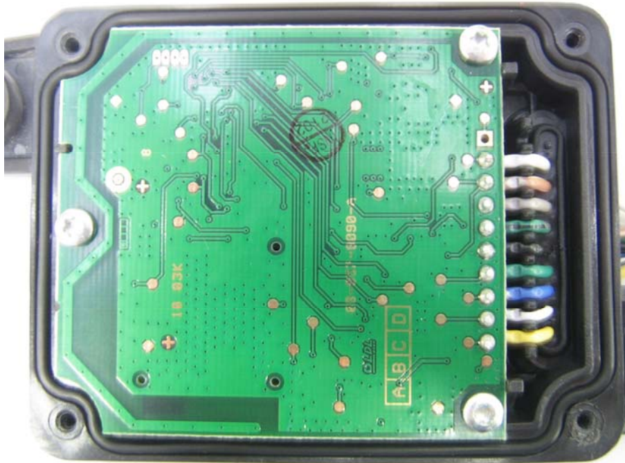
RCU PCB Underside B
