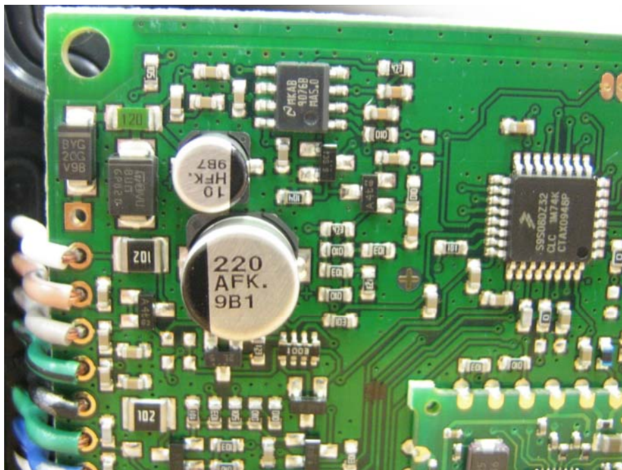
RC PCB Topside Upper Left Quadrant
