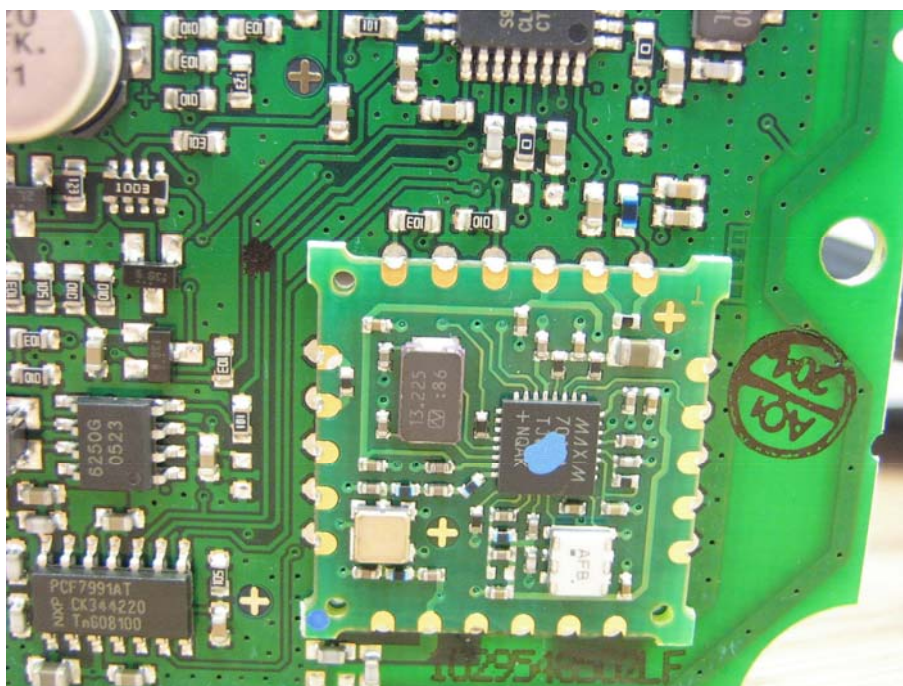
RC PCB Topside Lower Right Quadrant
