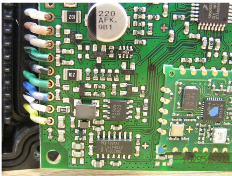
RC PCB Topside Lower Left Quadrant
