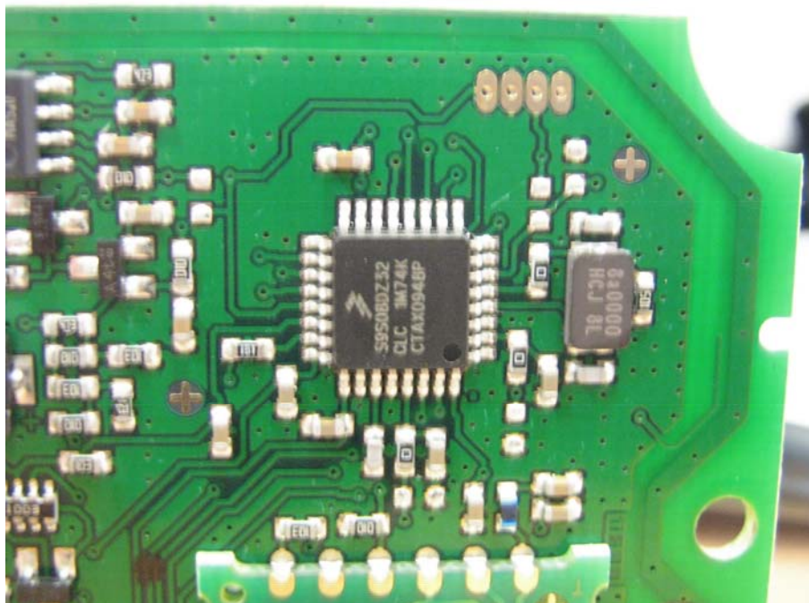
RC PCB Topside Upper Right Quadrant
