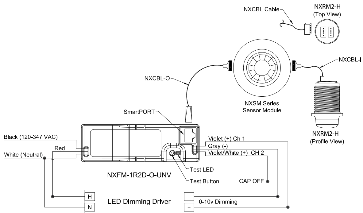
NXRM2-H with Sensor Figure 3
