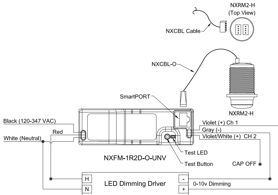
NXR2M2-H without Sensor
