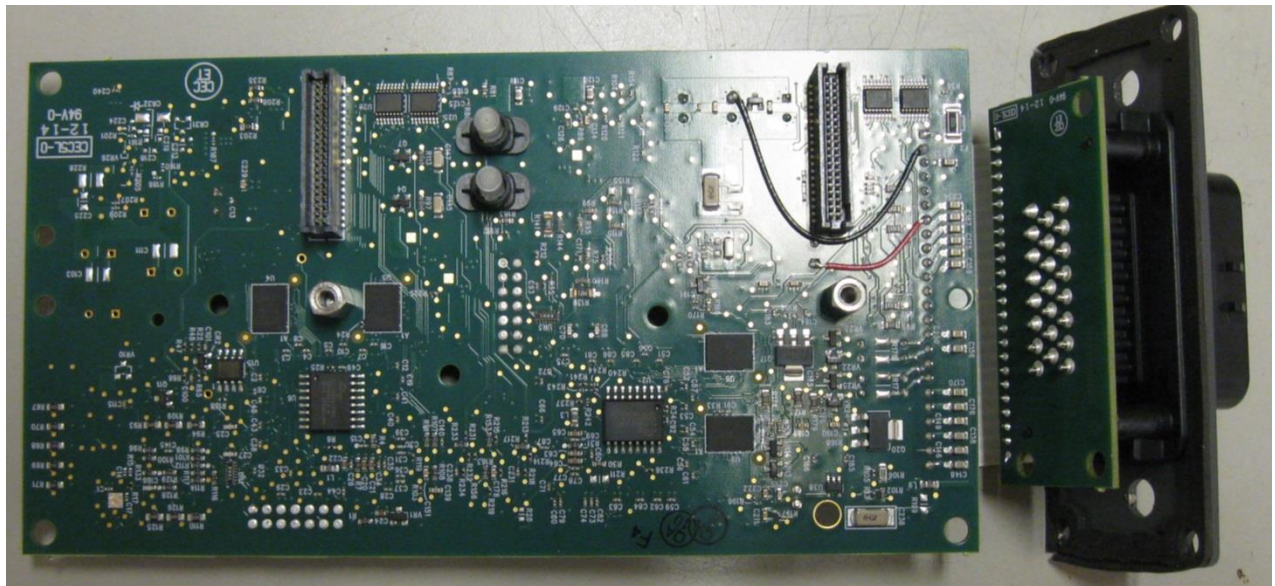
Main Board – connector side
