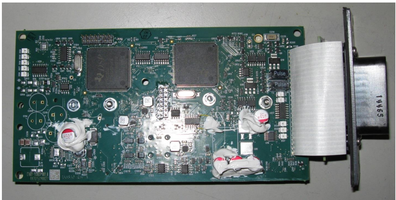
Main Board – Processor Side
