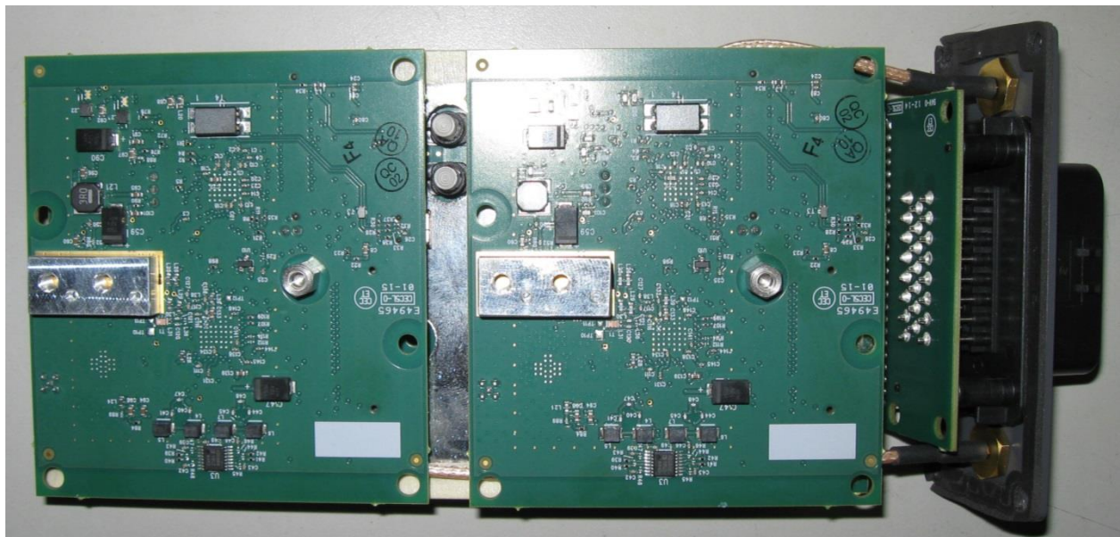
Assembled Antenna Board side
