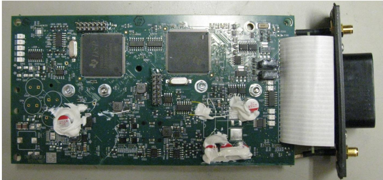
Assembled – processor side
