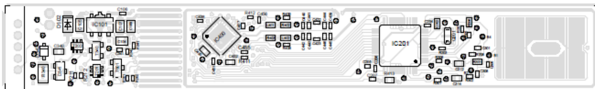
Figure 1: PCBA Kessy + NFC (Placement top)
