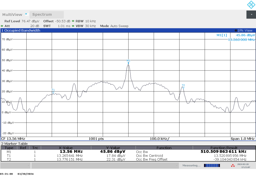
Plot no. 14: Frequency tolerance @ -40 °C, EUT A, Vmin
