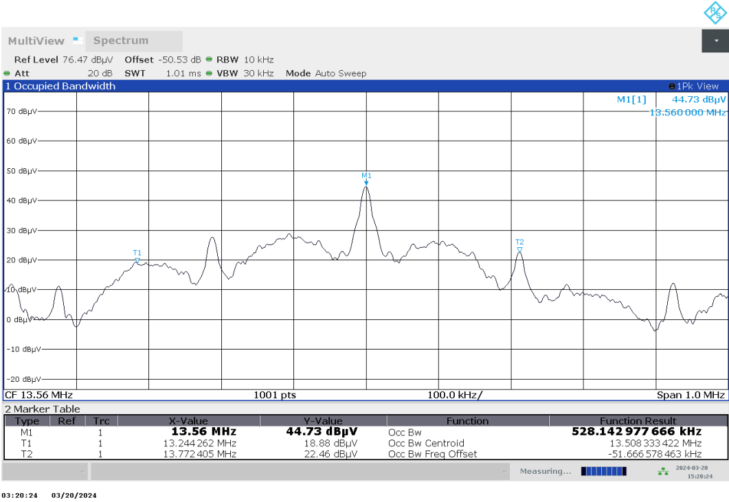
Plot No. 19: 99% Occupied bandwidth
