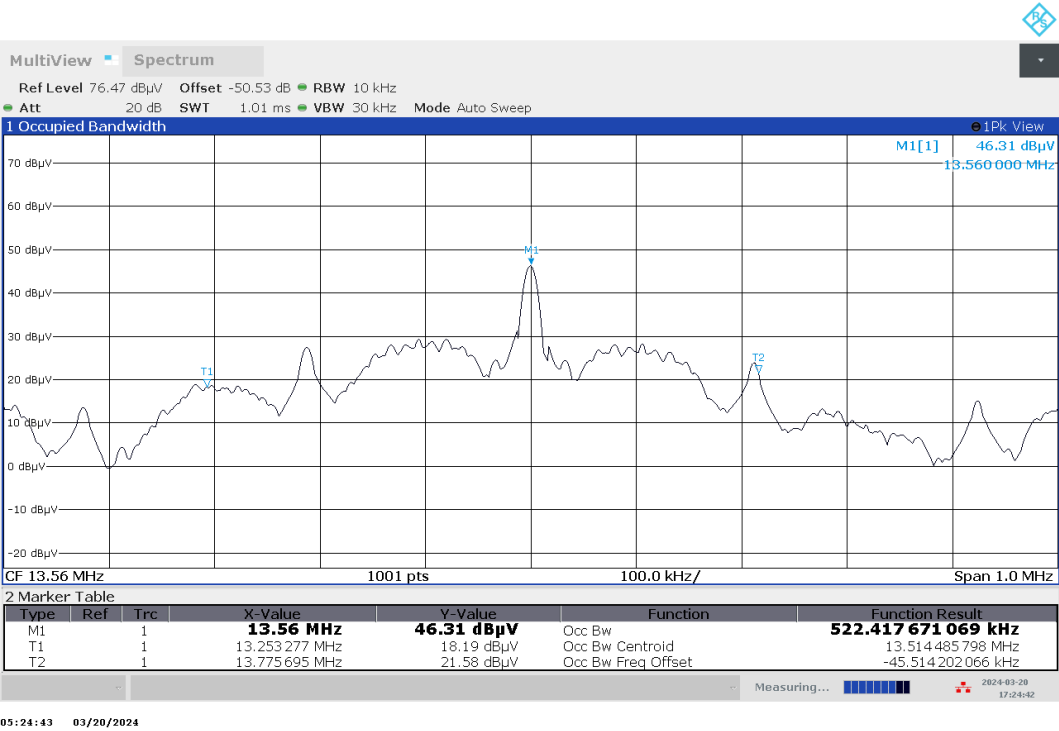
Plot no. 15: Frequency tolerance @ -40 °C, EUT A, Vmax
