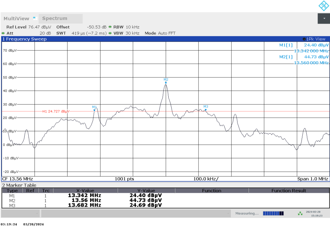
Plot No. 20: 20 dB bandwidth
