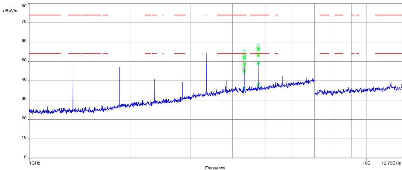
Plot 5: 1000 MHz to 12.75 GHz, vertical & horizontal polarisation, low channel
