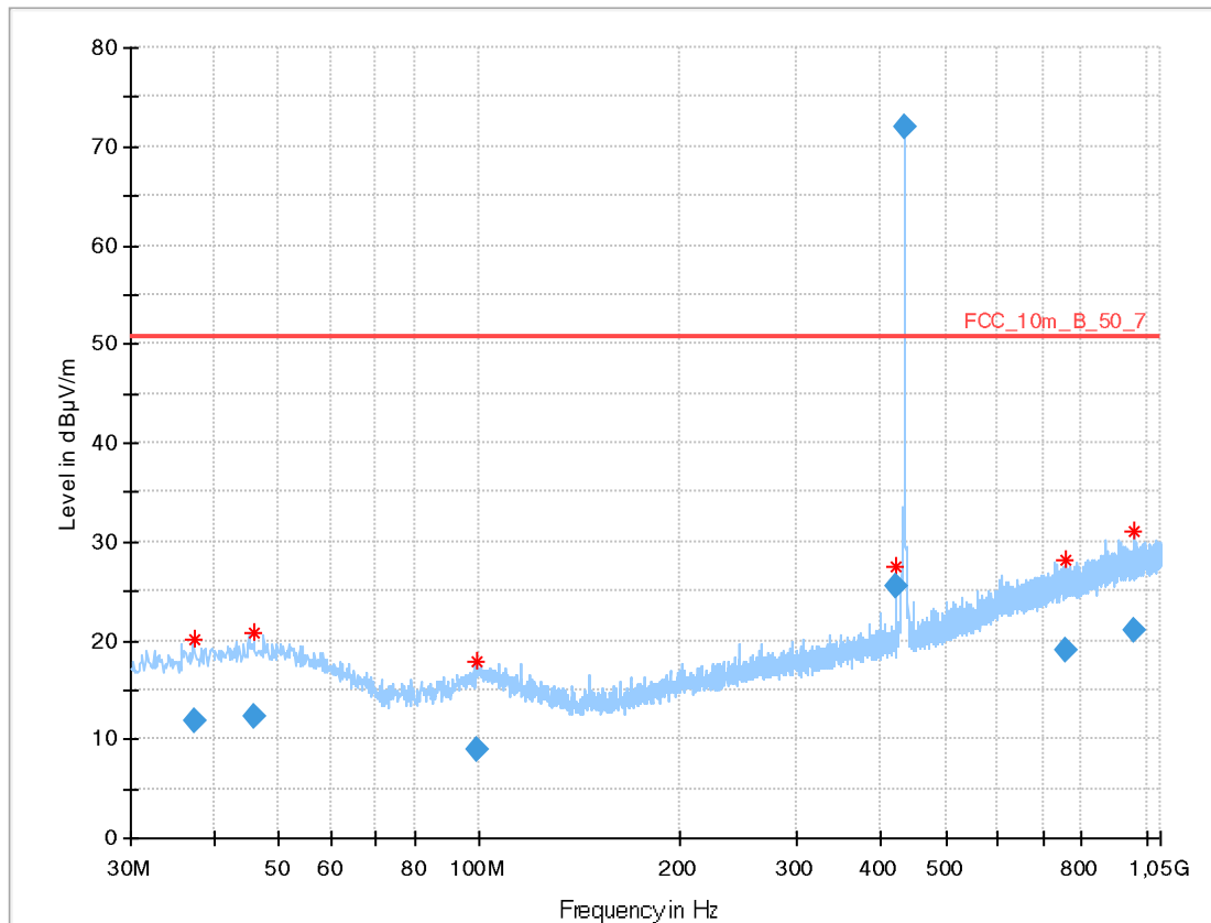
Plot 3: 30 MHz to 1000 MHz, vertical & horizontal polarisation, low channel
