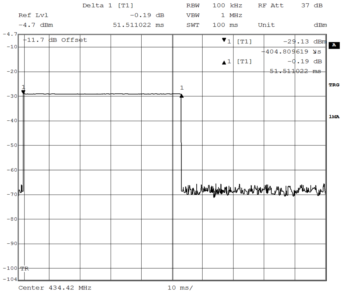
Fig. 2: Sweep to determine the "on" time within a 100 ms. After the command button is released, the EUT automatically stops transmitting in 52 ms.
