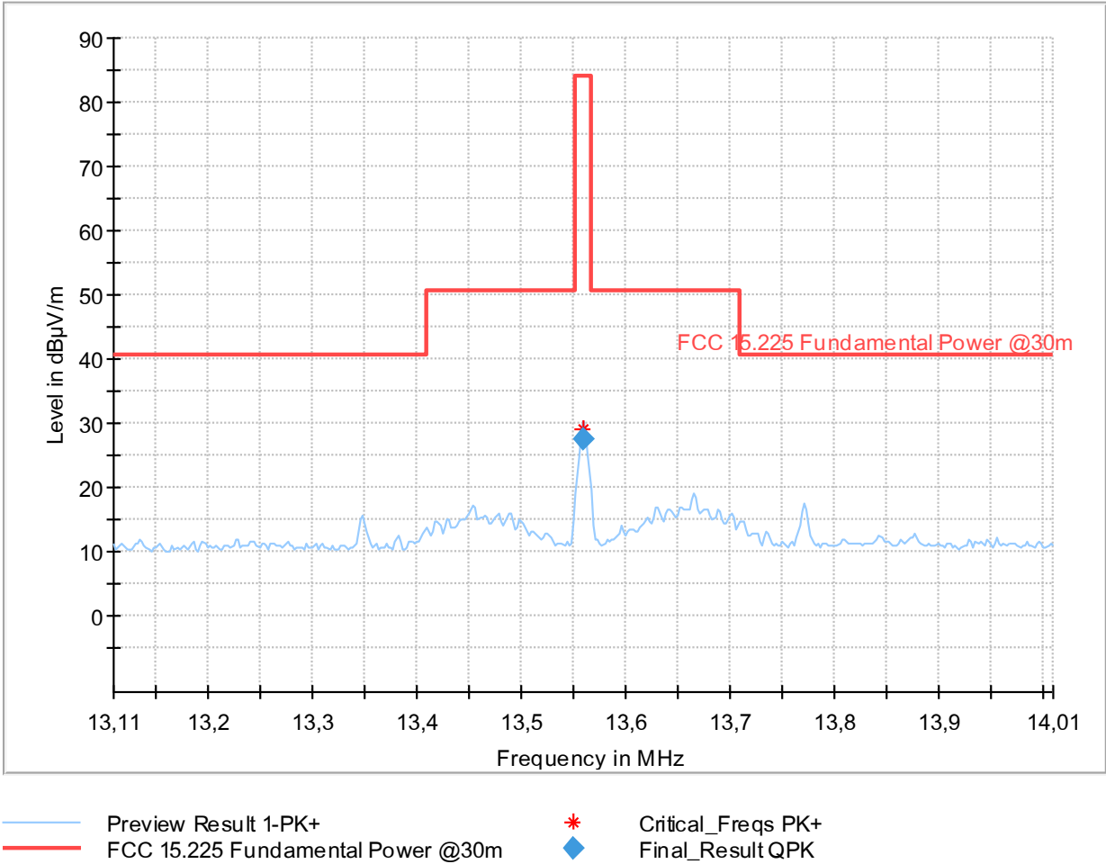
Plot no. 1: Transmitter Spectrum Mask (TSM)
