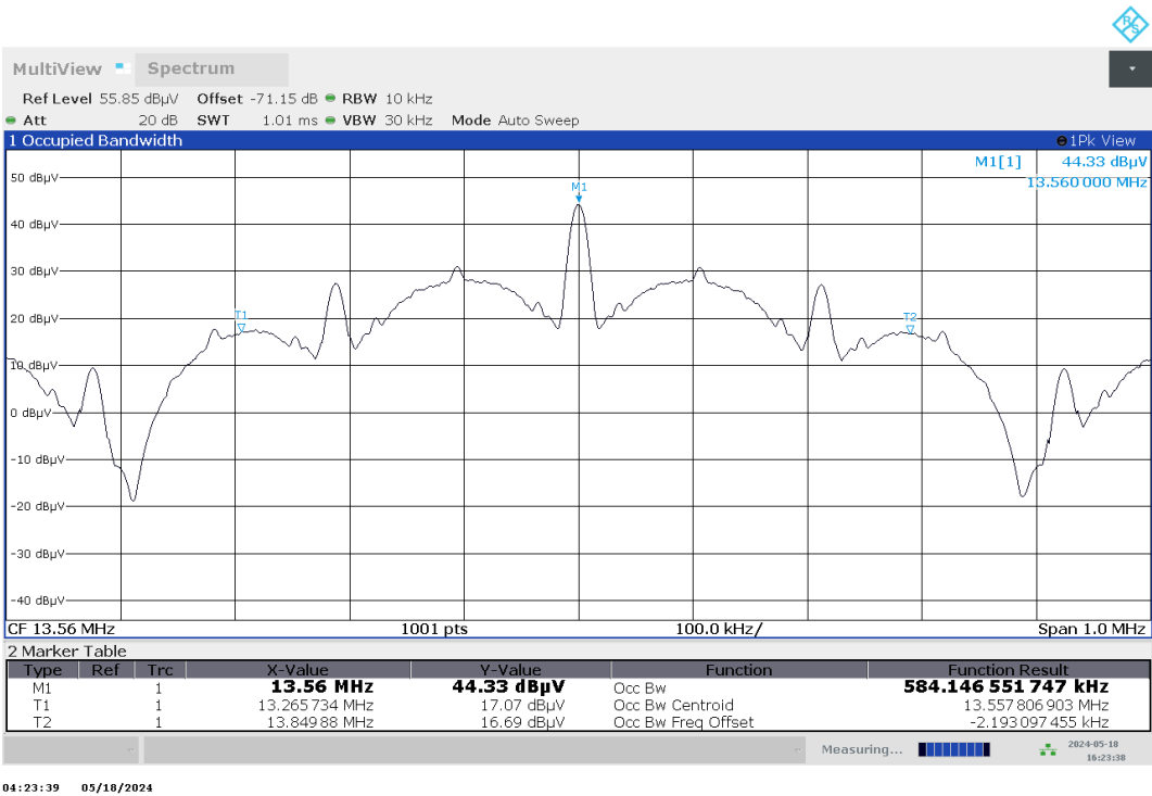
Plot no. 12: Frequency tolerance @ +85 C, EUT A, Vnom
