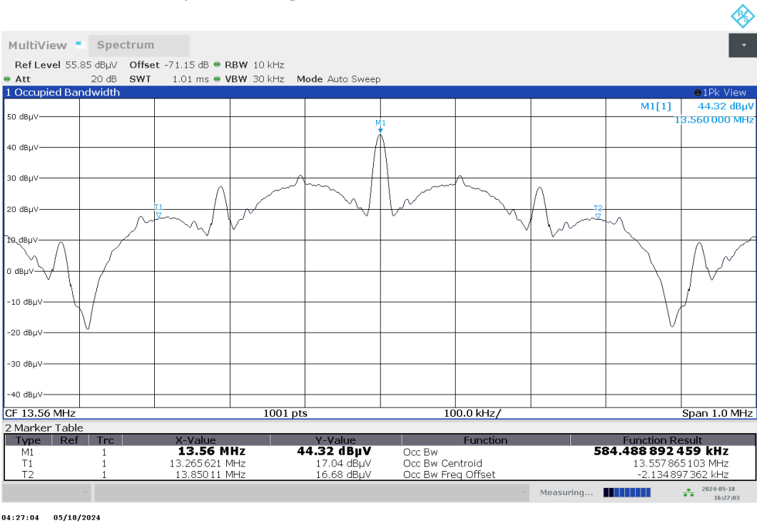
Plot no. 13: Frequency tolerance @ +85 C, EUT A, Vmin
