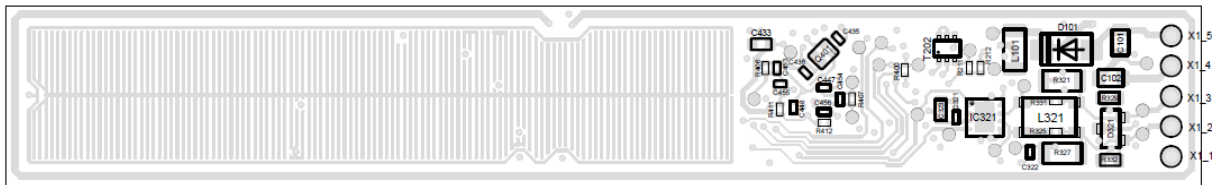
Figure 2: PCBA Kessy + NFC (Placement bottom)
