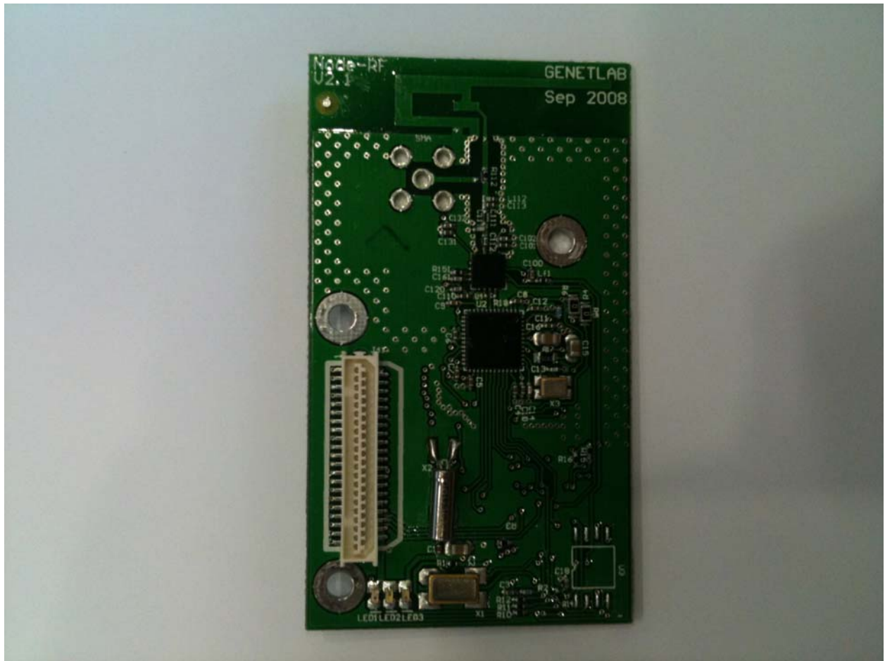
ClimateMinder Internal Photos of Wireless Radio Module FRONT
