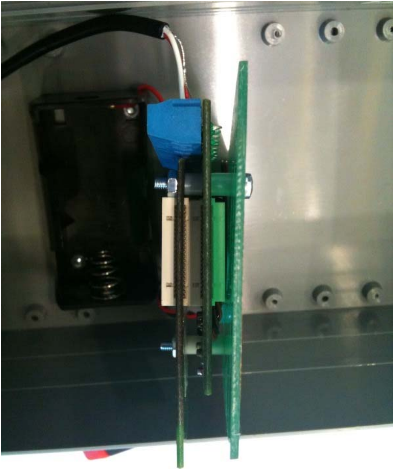
Radio module with Node Card – addl view
