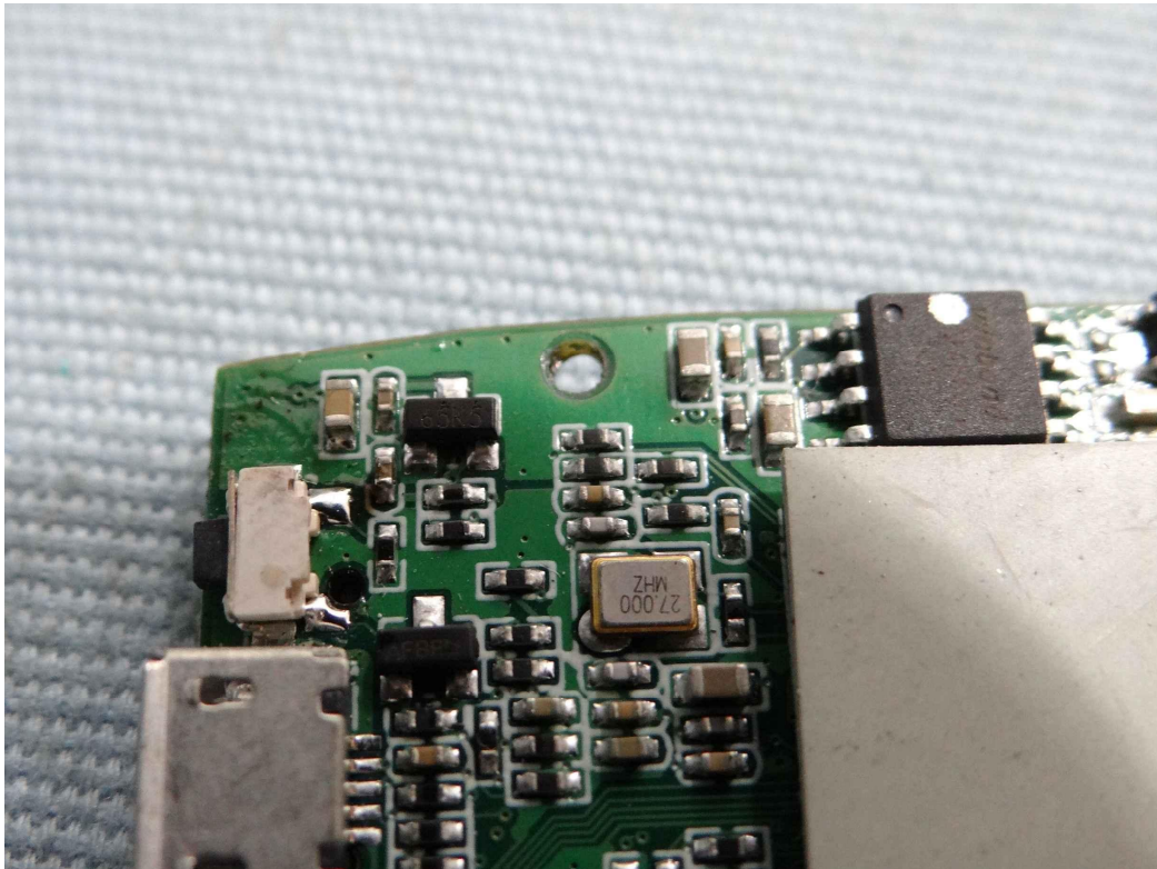
Y1 Crystal
