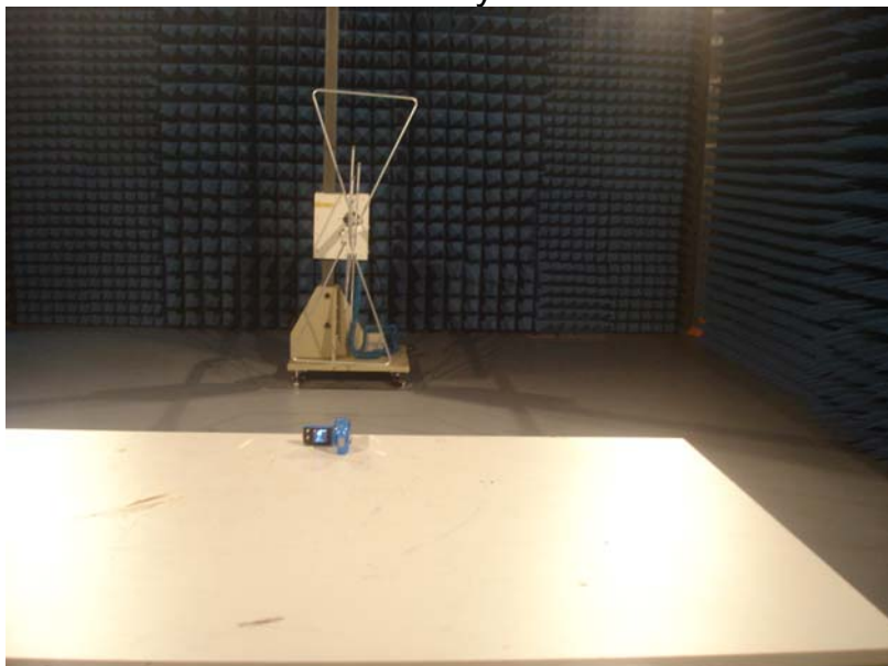
Photo of Setup for Radiated Emission Mode: Video record & Play back
