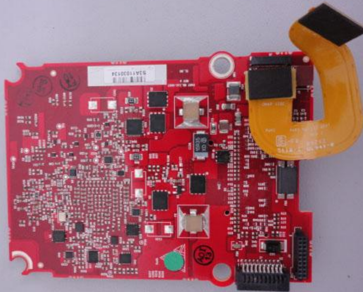
Bottom Side, OMAP Board
