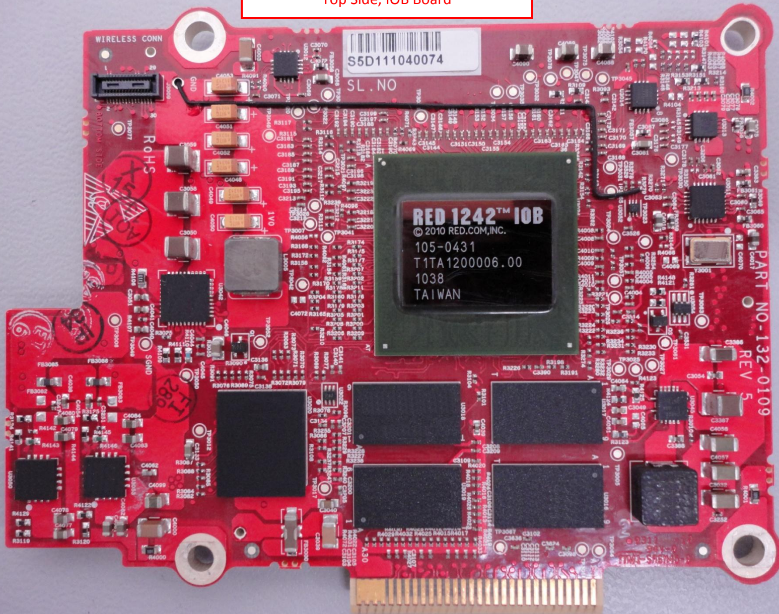
Top Side, IOB Board
