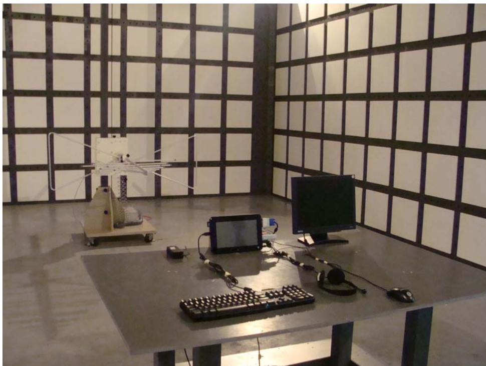
Radiated Emissions:
