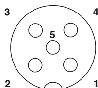
Figure 31 Power-OUT (X1), M12 female, A-coded
