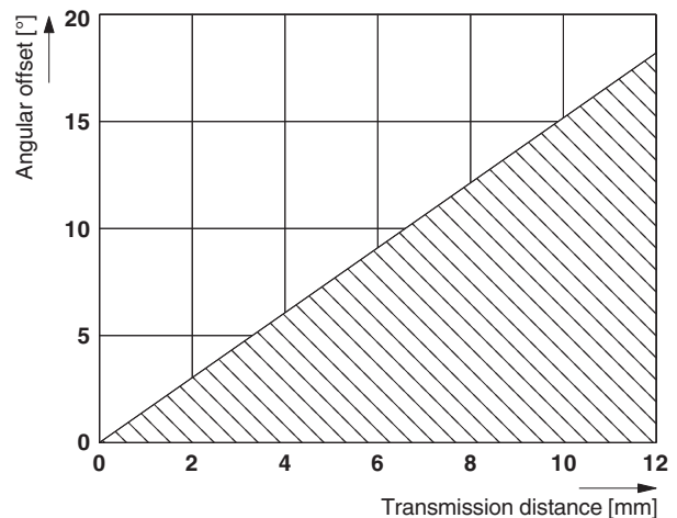
Figure 14 Transmission distance for angular offset, NEARFI PD...
