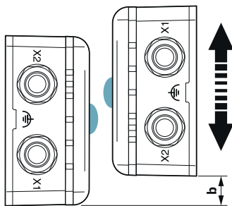
Figure 11 Lateral offset
