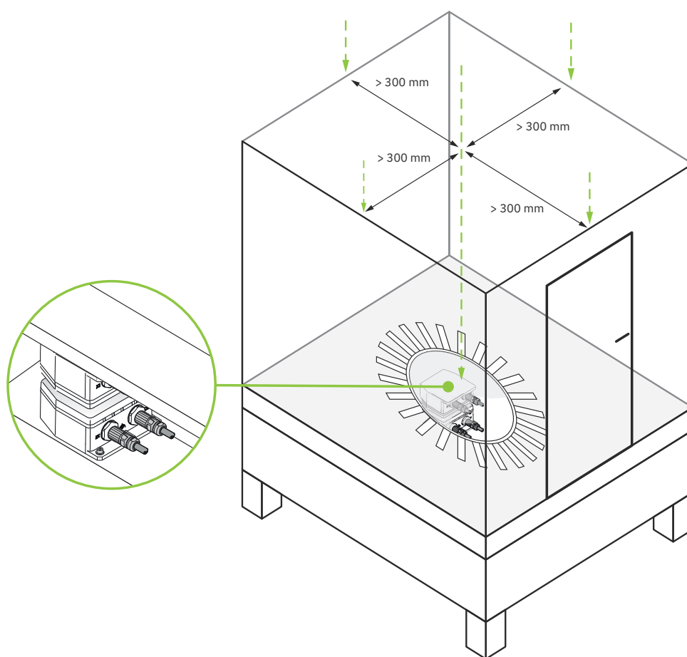
Figure 2 Rotary table
