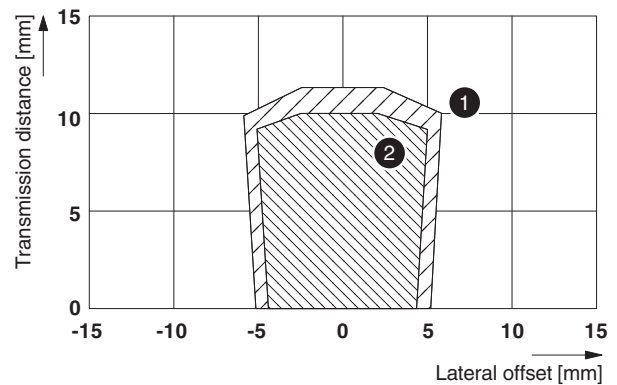
Figure 13 Transmission distance for lateral offset, NEARFI PD...
