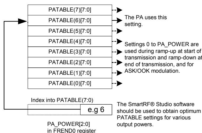
Figure 27: PA_POWER and PATABLE
