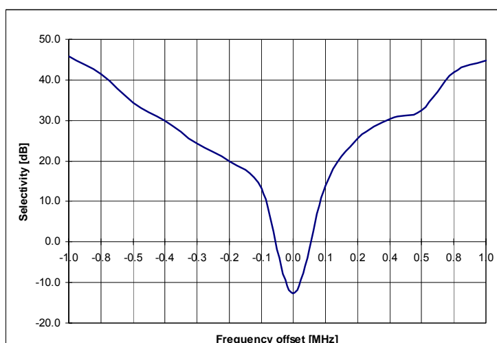
Figure 3: Typical Selectivity at 38.4 kBaud Data Rate, 868 MHz, GFSK, 20 kHz Deviation. IF Frequency is 152.3 kHz and the Digital Channel Filter Bandwidth is 100 kHz
