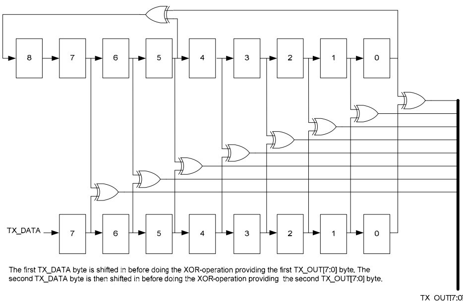
Figure 15: Data Whitening in TX Mode
