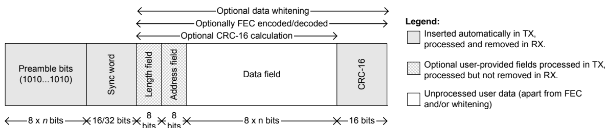
Figure 16: Packet Format
