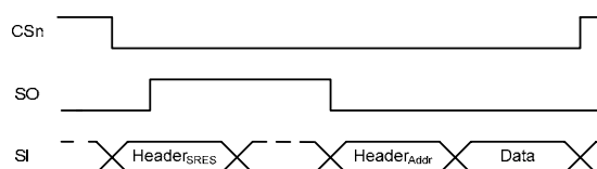
Figure 13: SRES Command Strobe
