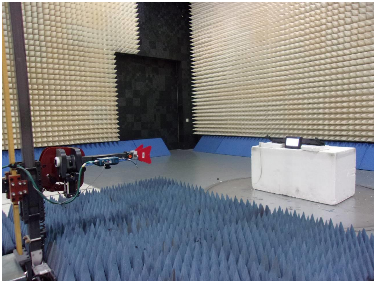
Figure 2 FCC Title 47 CFR Part 15B Radiated Emissions 1 – 18GHz
