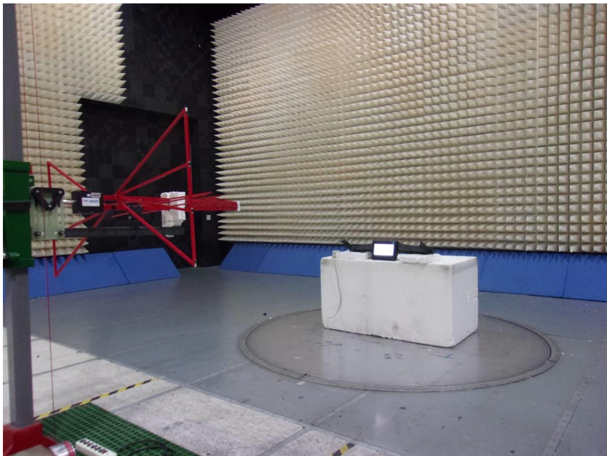
Figure 1 Radiated emissions, 30 MHz – 1 GHz
