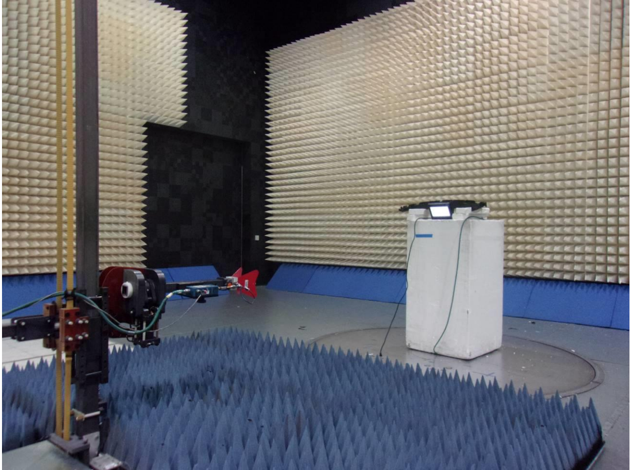
Figure 3 FCC Title 47 CFR Part 22, 24, 27, 90 Radiated Spurious Emissions 1 – 18 GHz
