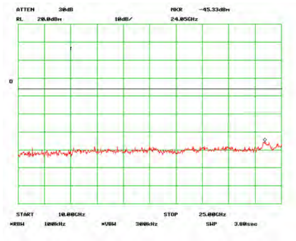
Antenna Port Emission Low-4
