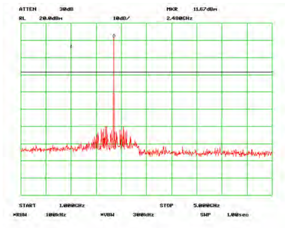
Antenna Port Emission High-2
