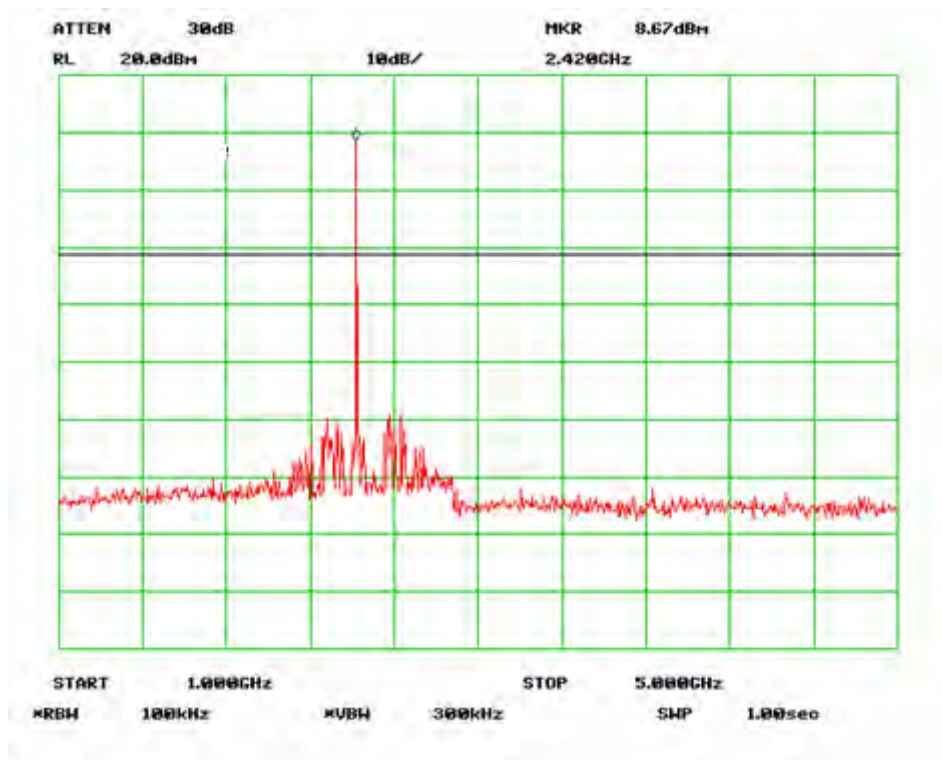
Antenna Port Emission Mid-2
