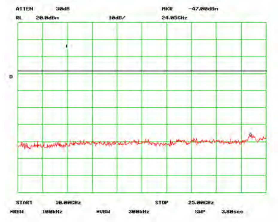
Antenna Port Emission High-4
