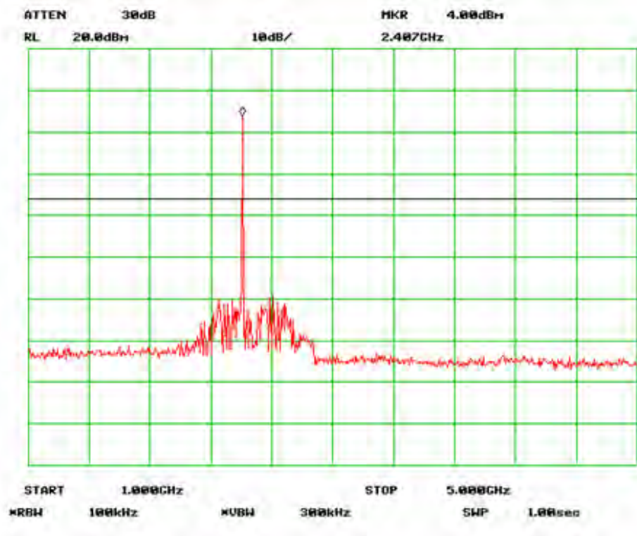
Antenna Port Emission Low-2
