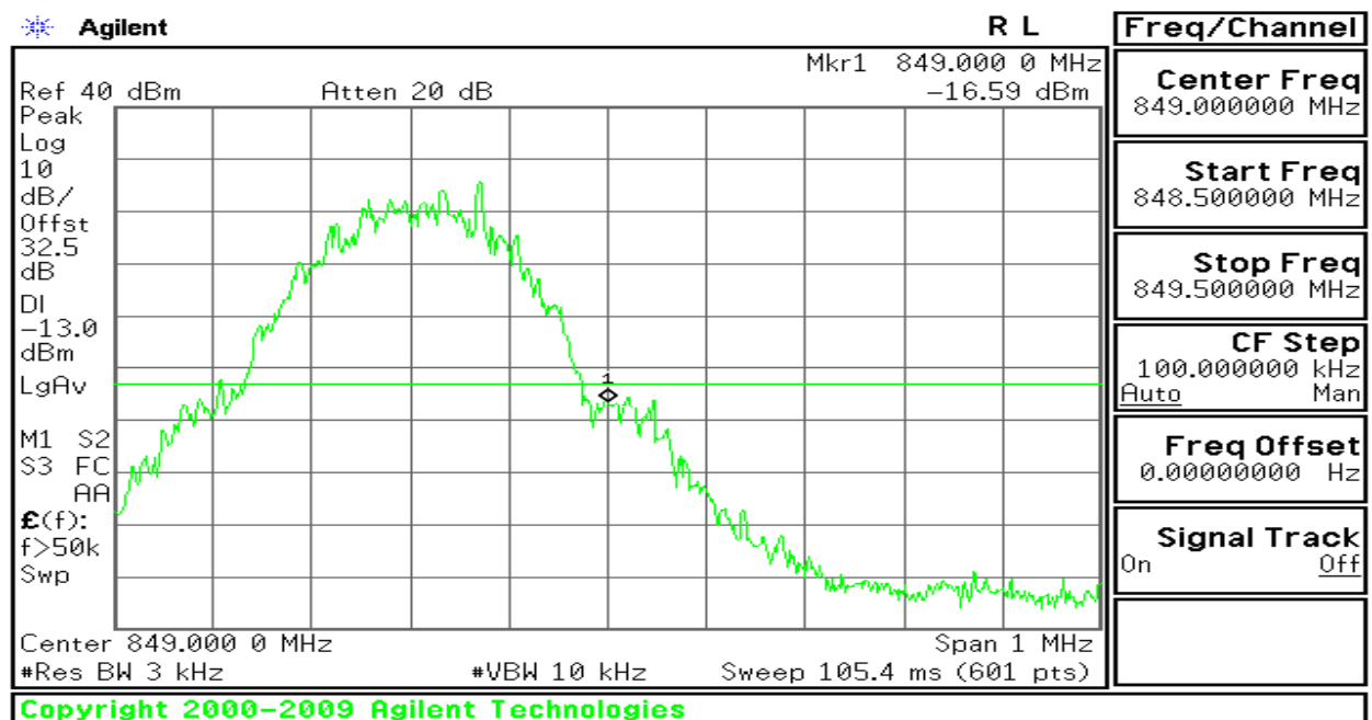
Figure 9-2: Band Edge emissions – GSM CH High
