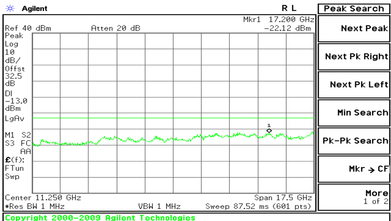
Figure 7-6: Out of Band emission at antenna terminals – GSM CH High
