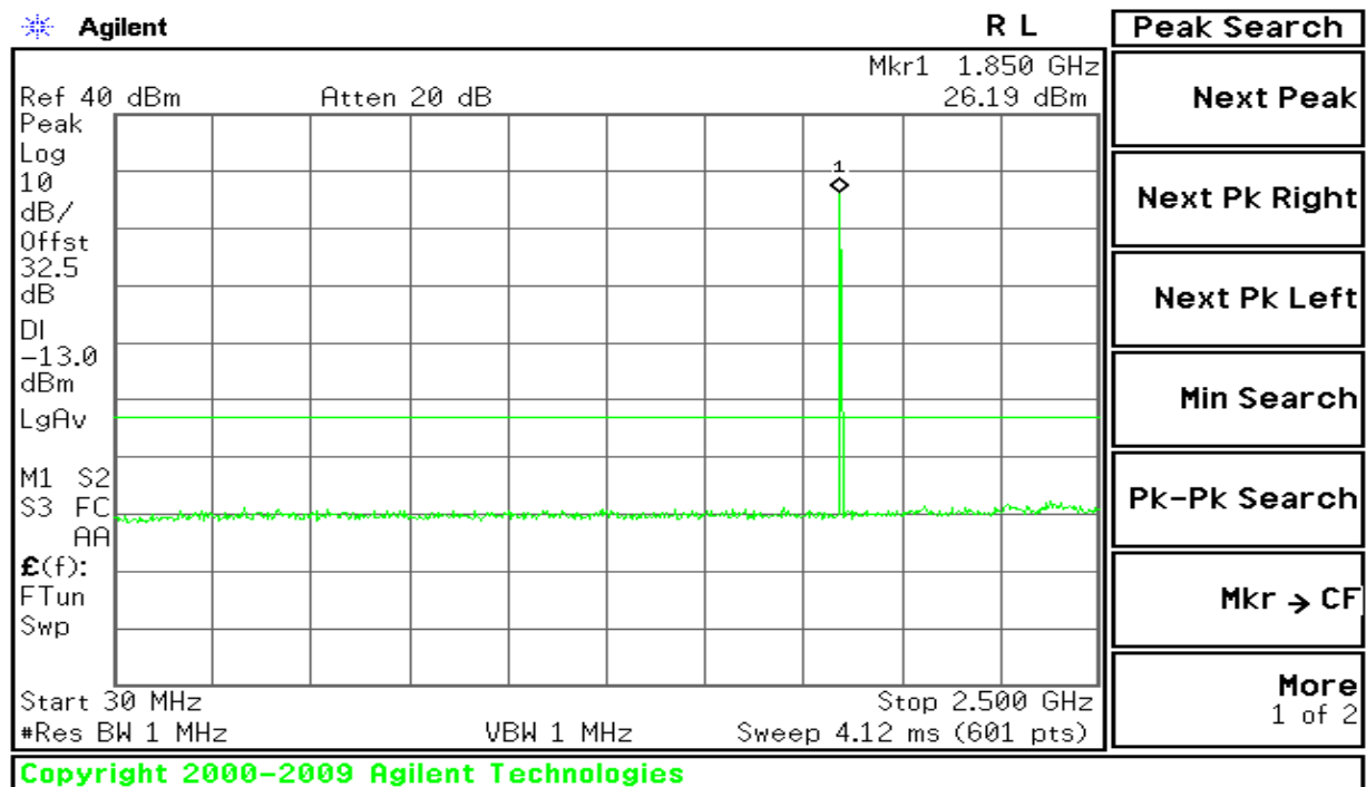
Figure 8-1: Out of Band emission at antenna terminals – GSM CH Low
