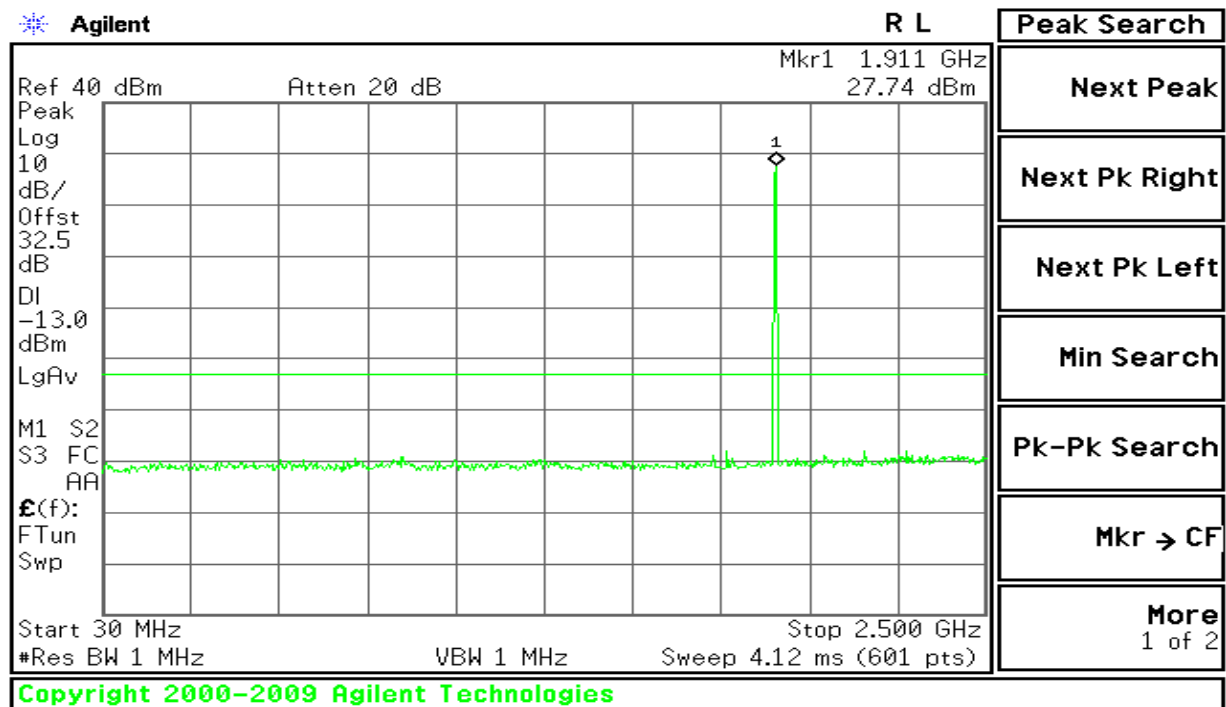
Figure 8-5: Out of Band emission at antenna terminals – GSM CH High
