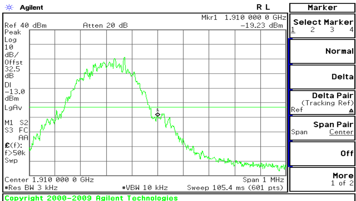
Figure 10-2: Band Edge emissions – GSM CH High
