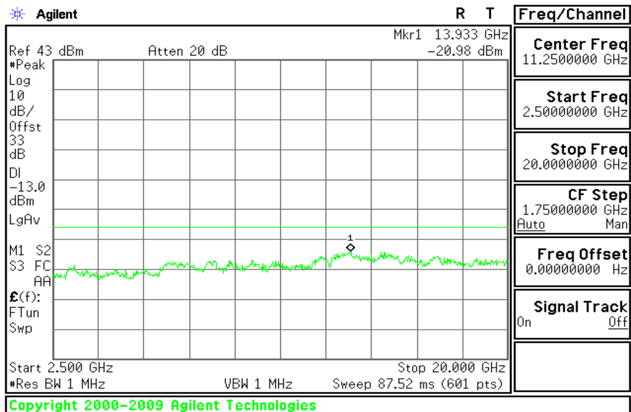
Figure 8-10: Out of Band emission at antenna terminals – GPRS CH Middle
