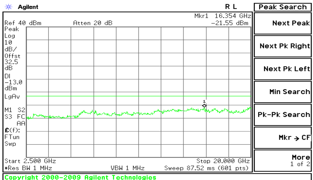
Figure 8-6: Out of Band emission at antenna terminals – GSM CH High
