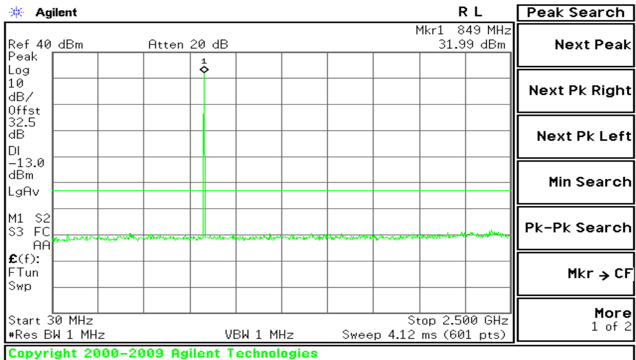
Figure 7-5: Out of Band emission at antenna terminals – GSM CH High
