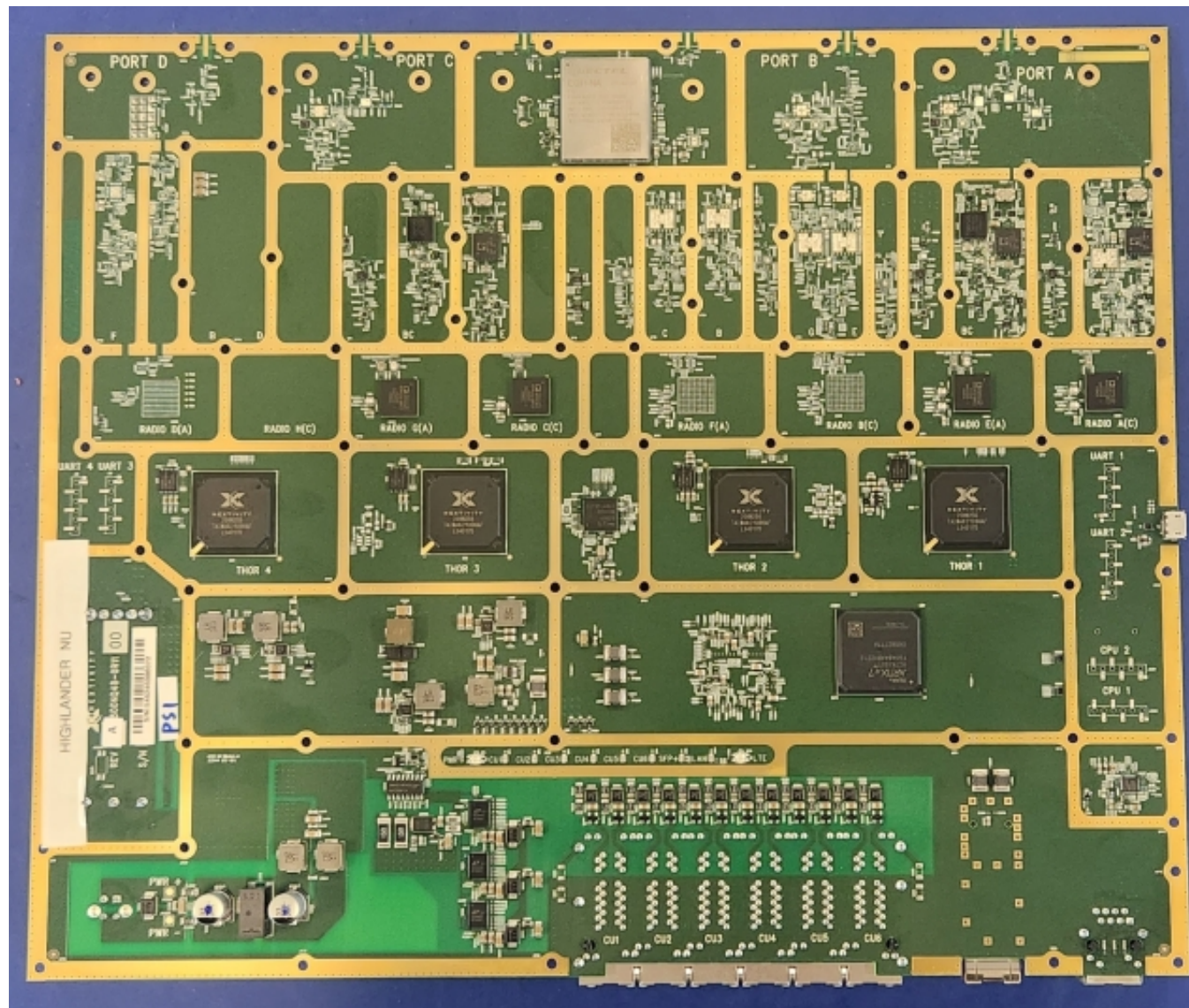
PCB side 1
