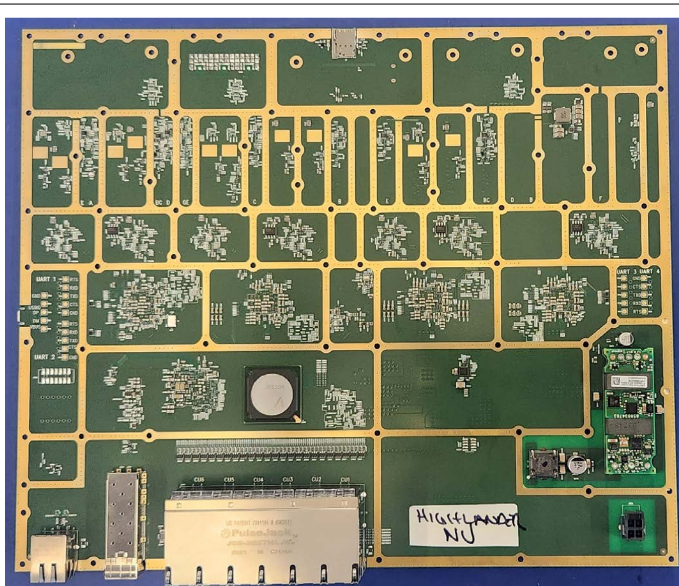
PCB side 2
