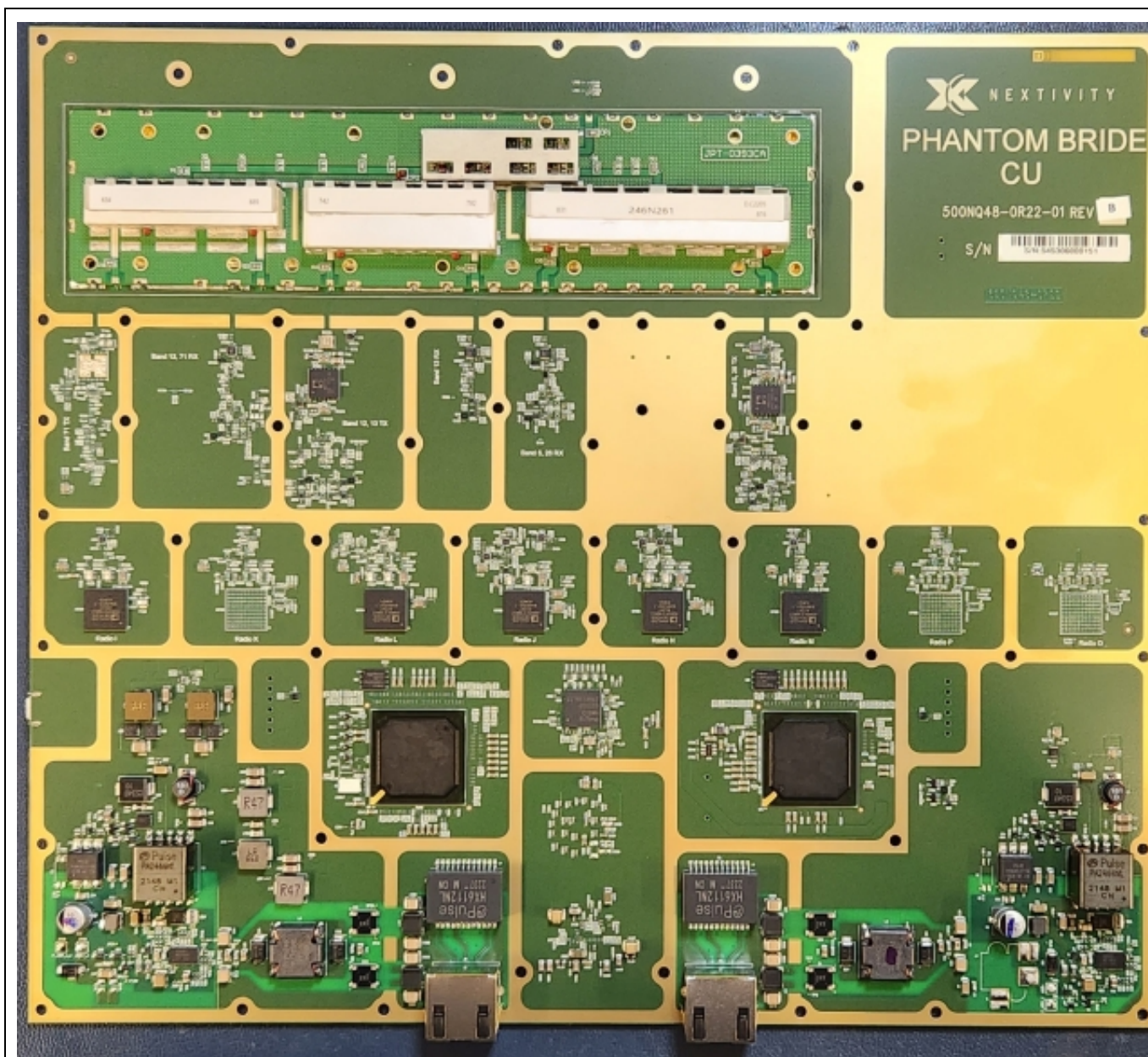
PCB side 2
