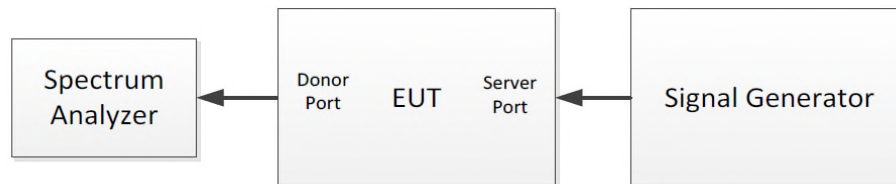
Figure 2 – Uplink test configuration in EUT test mode
