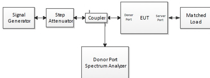
Figure 7 – Uplink RSSI-dependent noise limit test configuration
