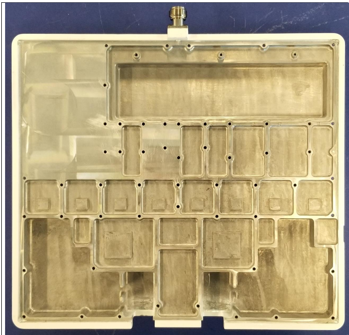
Housing_Bottom_Internal
