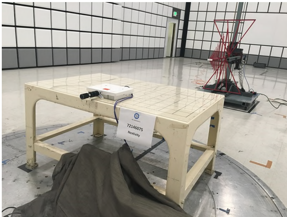
CU Radiated Emissions Below 1GHz Rear
