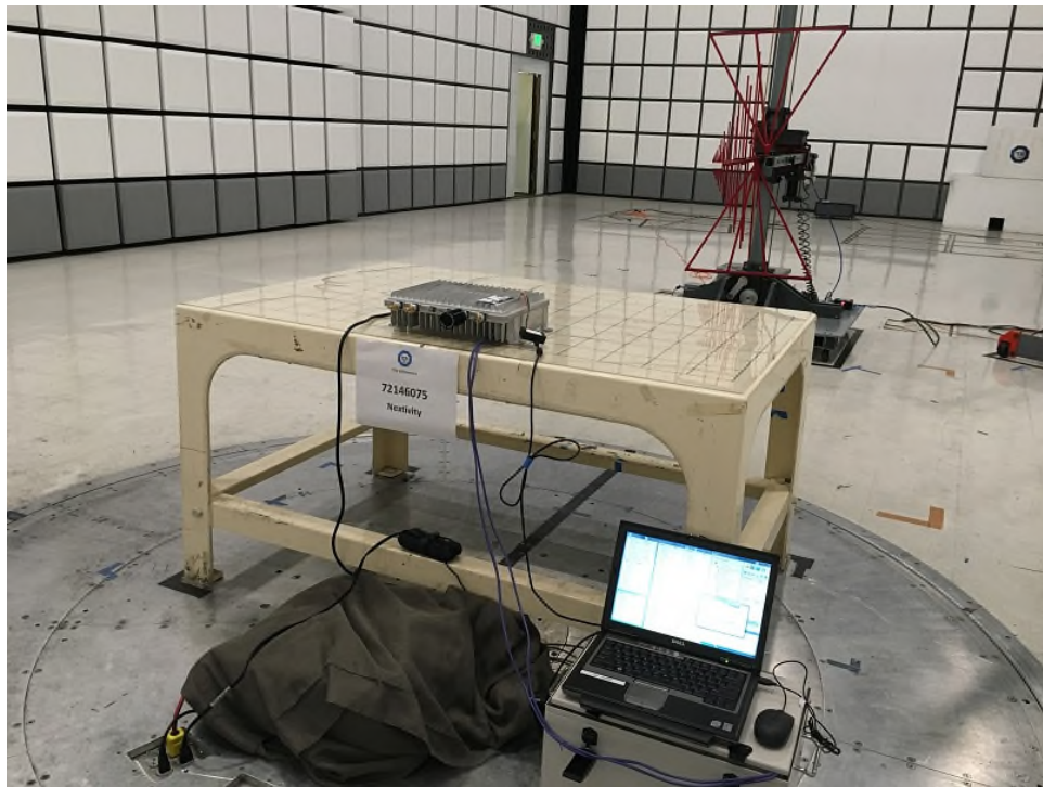
NU Intermodulation Radiated Emissions Below 1GHz Rear
