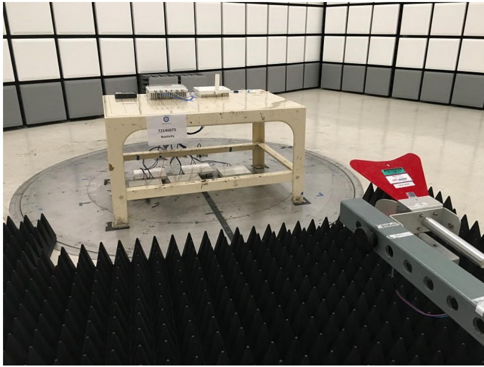
NU Radiated Emissions Above 1GHz Front (Unintentional)
