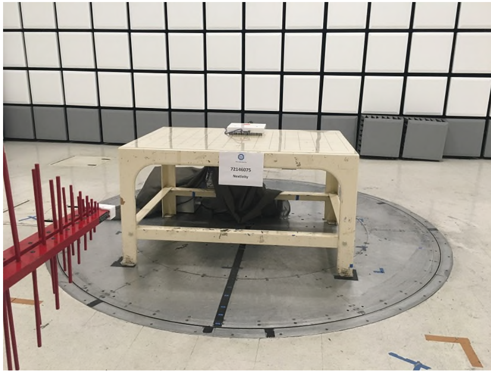
CU Intermodulation Radiated Emissions Below 1GHz Front
