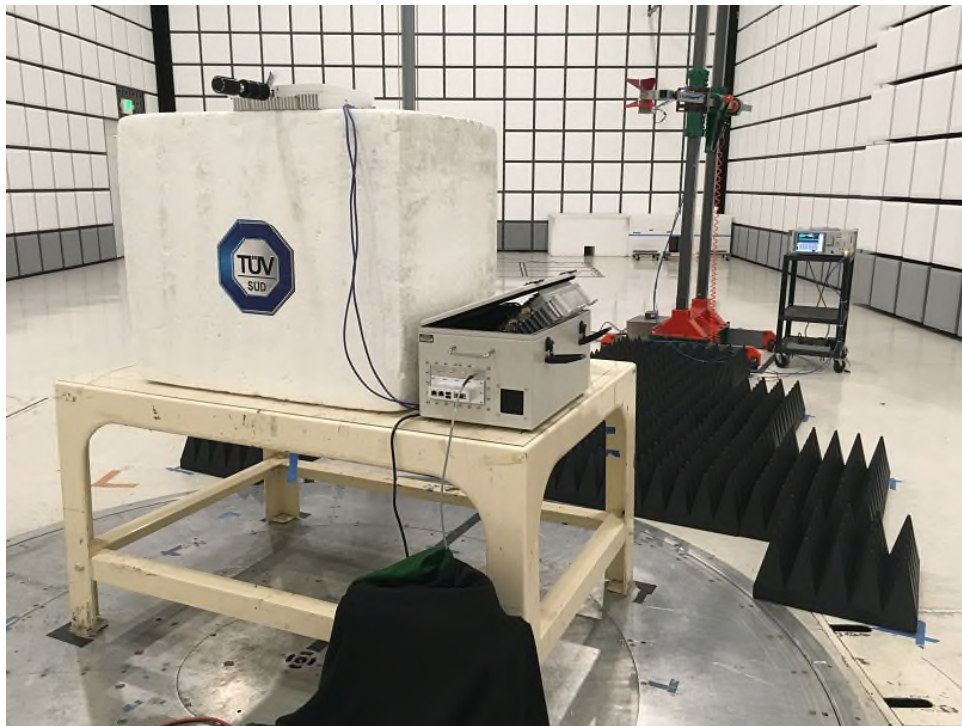
CU Intermodulation Radiated Emissions Above 1GHz Rear
