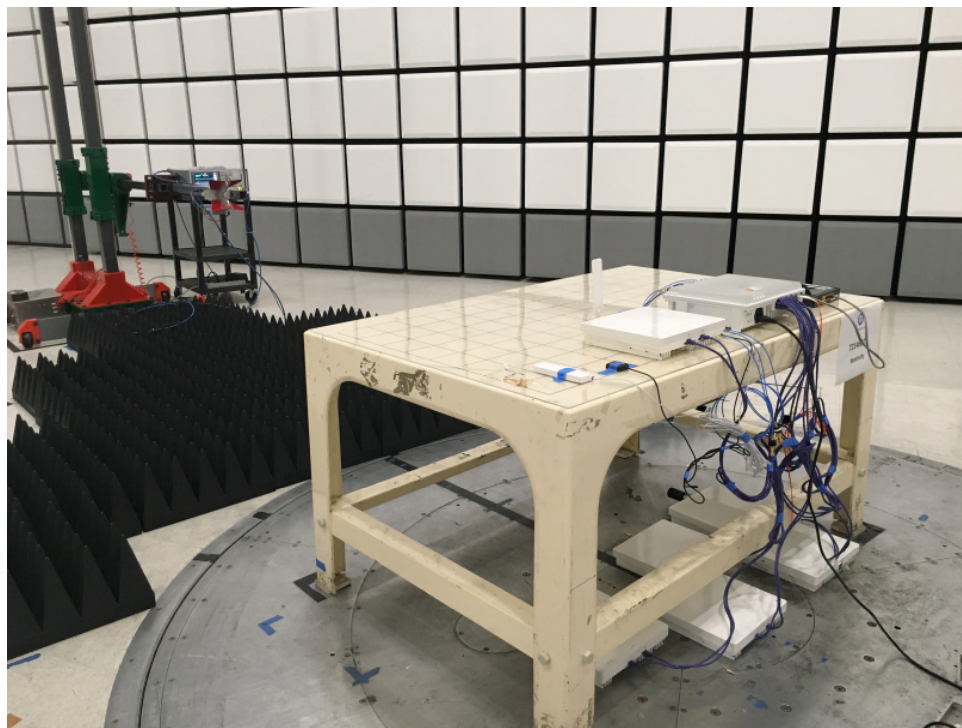
NU Radiated Emissions Above 1GHz 1GHz Rear (Unintentional)
