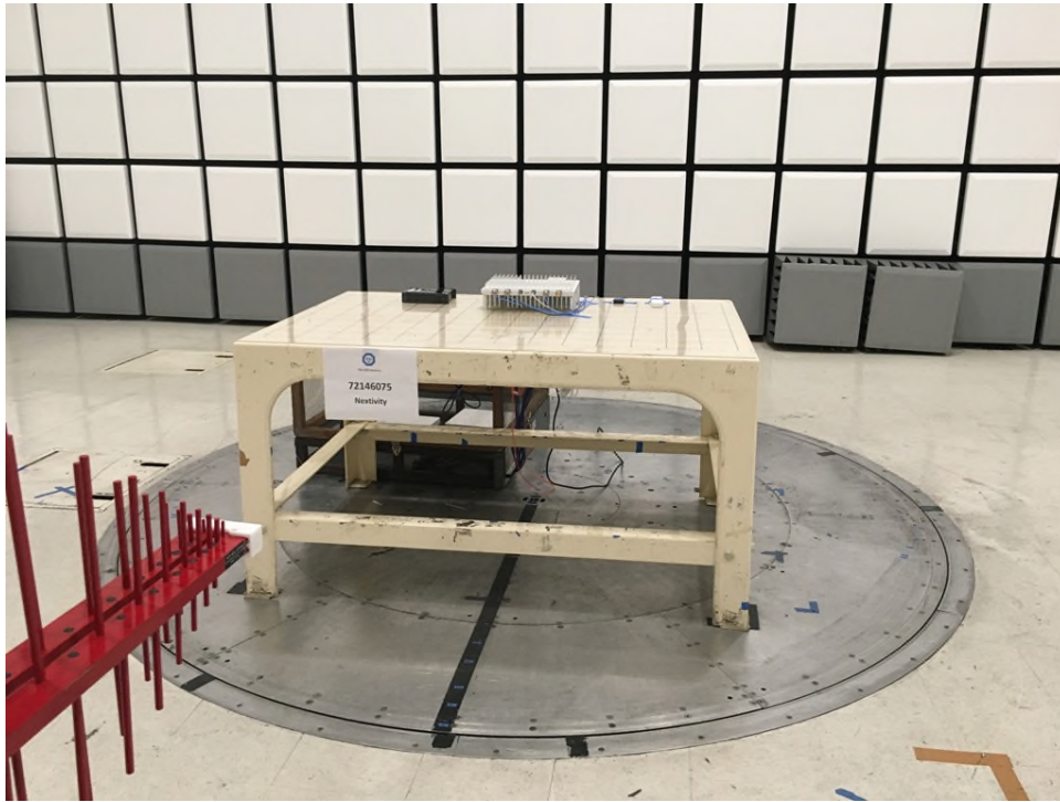
NU Radiated Emissions Below 1GHz Front (Unintentional)
