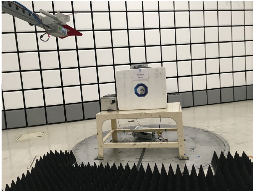
NU Intermodulation Radiated Emissions Above 1GHz Front
