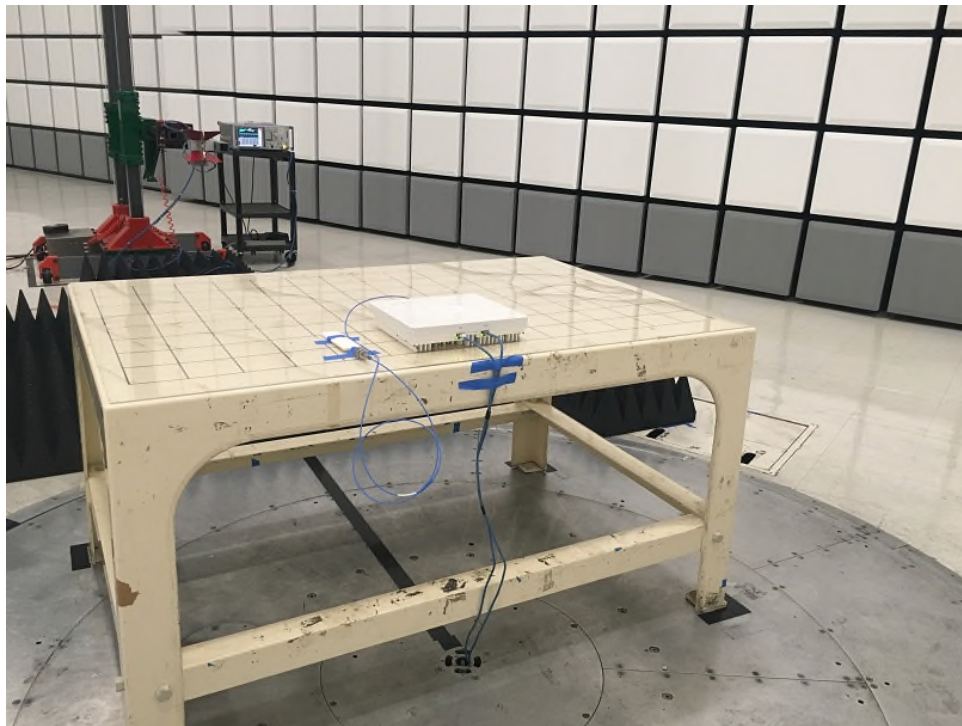
CU Radiated Emissions Above 1GHz Rear (Unintentional)
