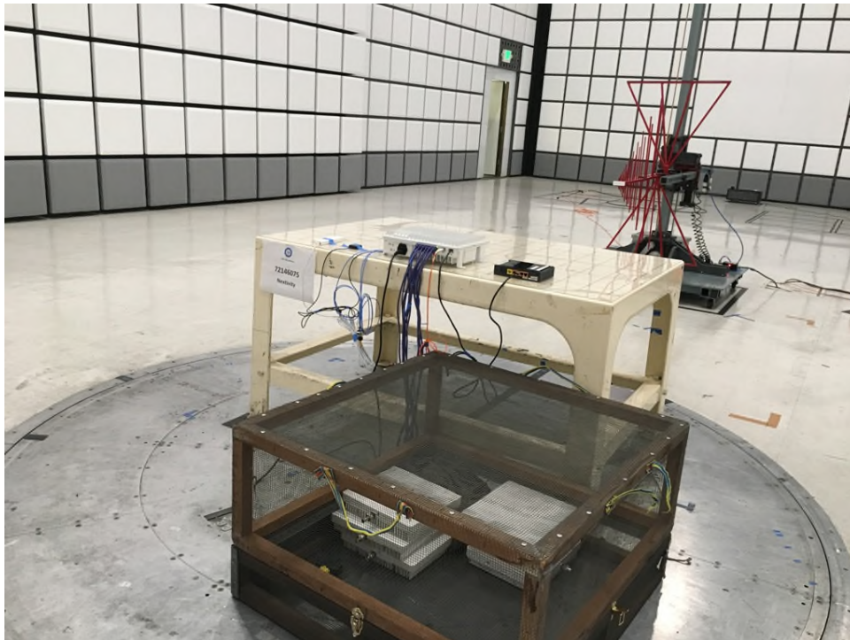
NU Radiated Emissions Below 1GHz Rear (Unintentional)
