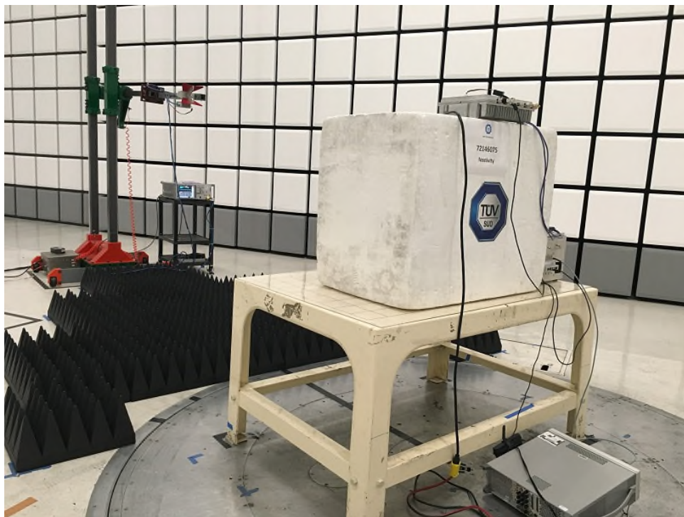
NU Intermodulation Radiated Emissions Above 1GHz Rear
