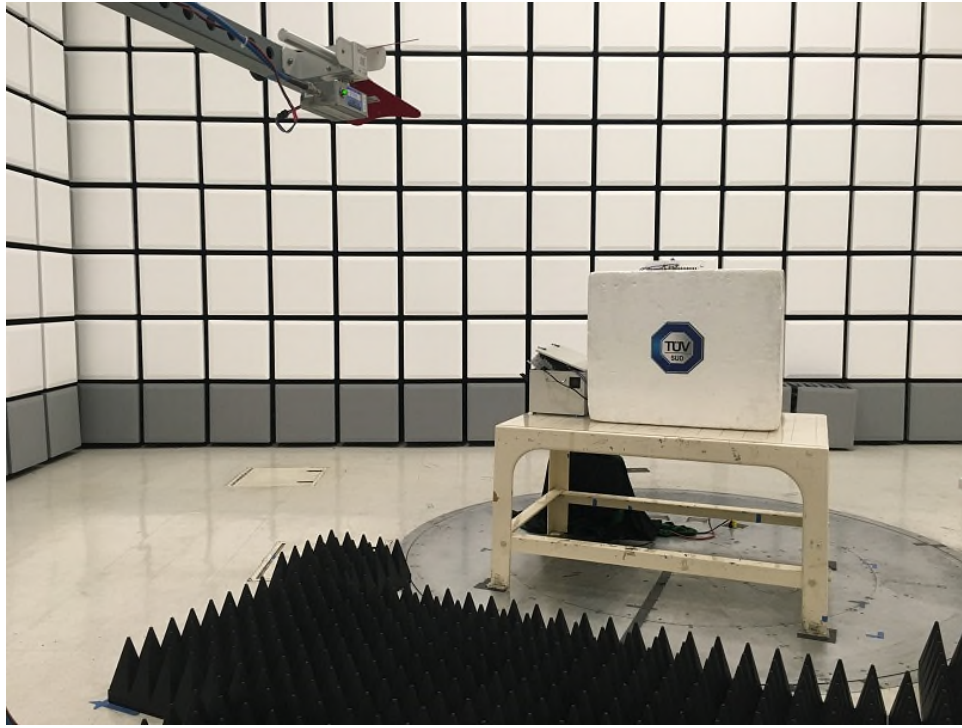
CU Intermodulation Radiated Emissions Above 1GHz Front
