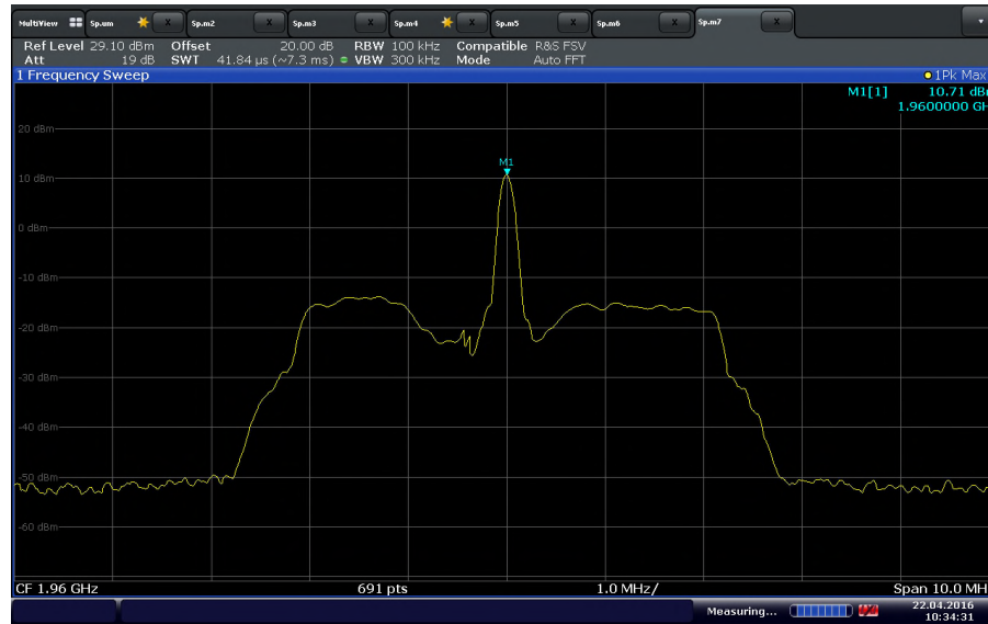
WCDMA B2 Downlink Mid Channel 120VAC @ 20°C
