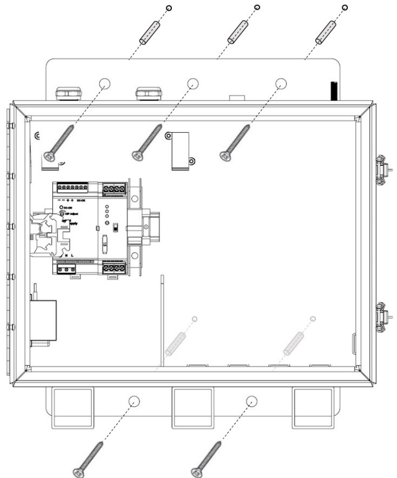
BBU Wall Mounting
