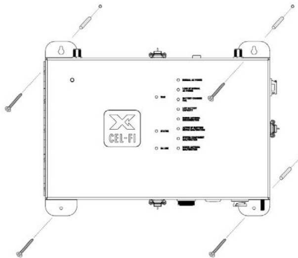
BDA Wall Mounting
