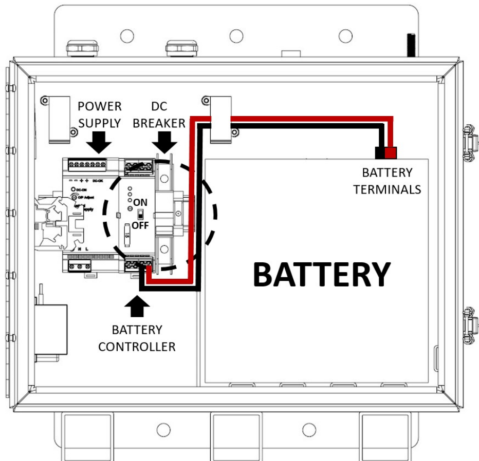
Battery connection scheme
