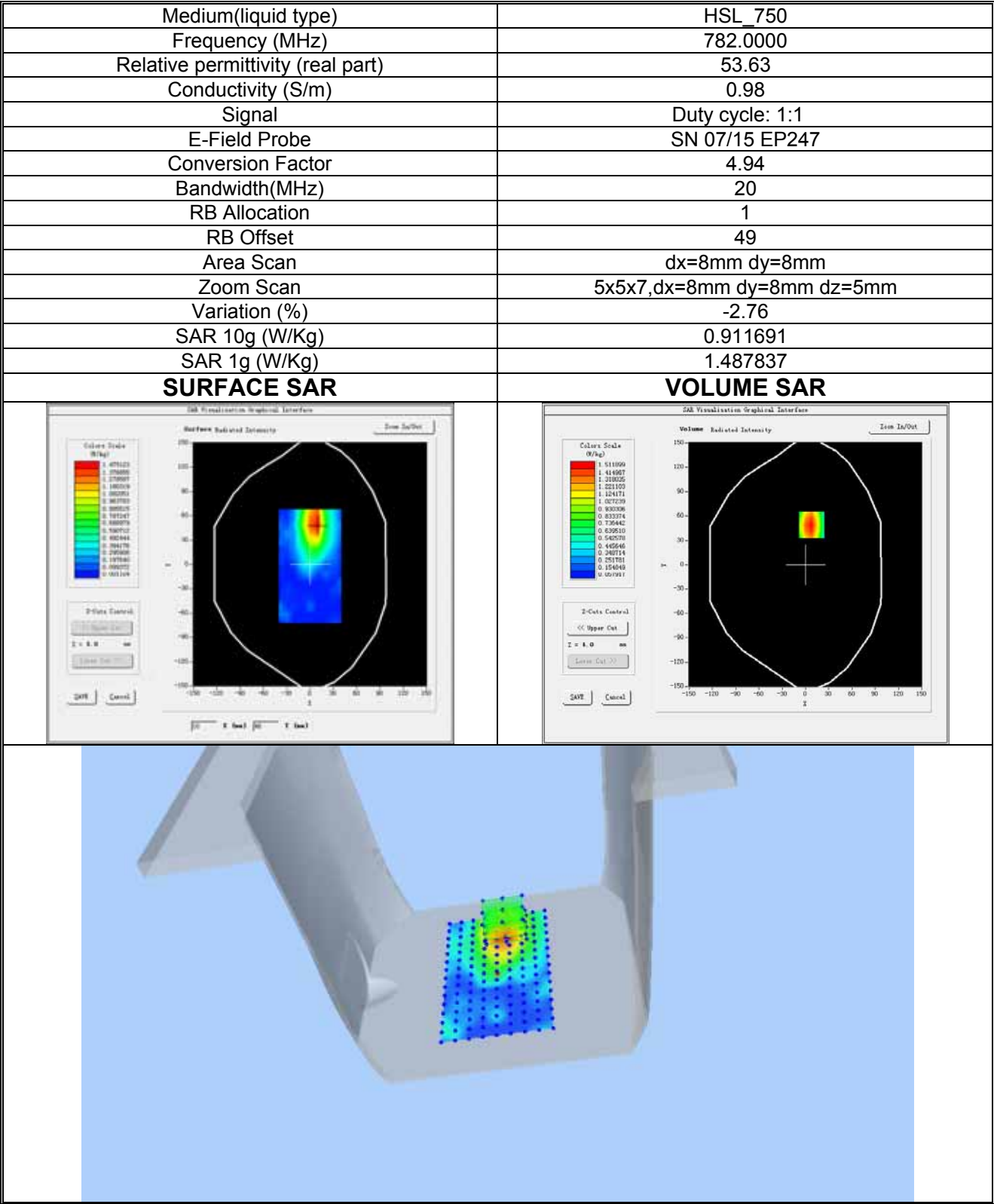
Plot 9:LTE BAND 13, Middle channel (Hotspot, Top Edge) Product Description:CEL FI COMPASS Test Date: 2019-12-13
