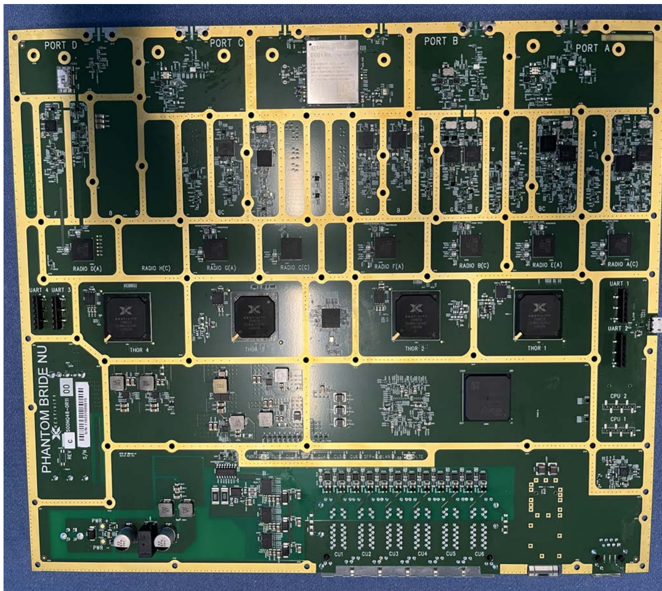
PCB side 1
