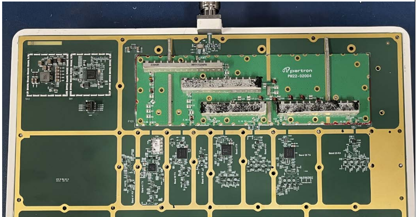
PCB Side 1_Radio
