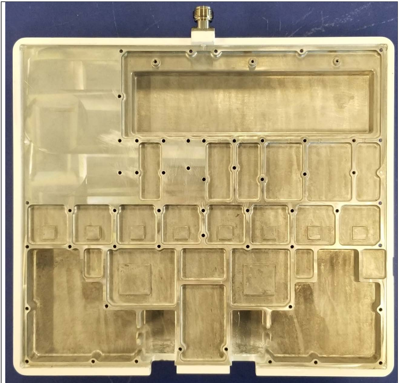
Housing_Bottom_Internal
