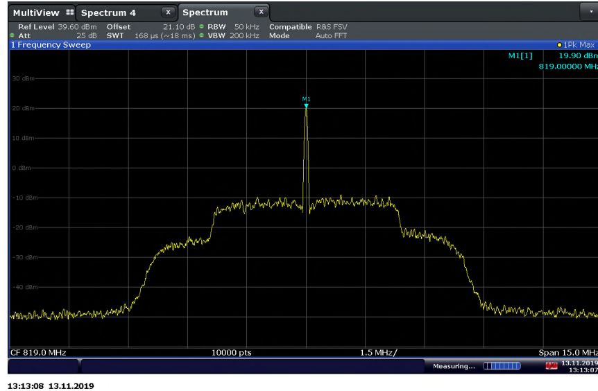
LTE Band 26 (814 – 849 MHz) Uplink 120VAC @ 20°C
