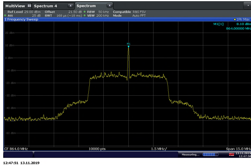
LTE Band 26 (859 – 869 MHz) Downlink 120VAC @ 20°C
