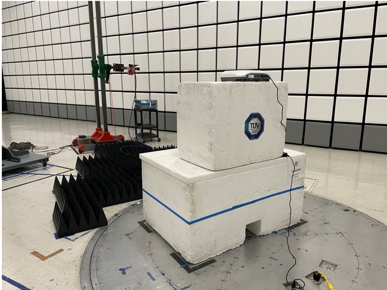
Radiated Spurious Emissions Test Setup 1GHz to 18GHz
