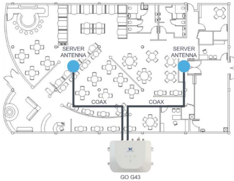
Two Server Antenna Ports, each feeding one antenna
