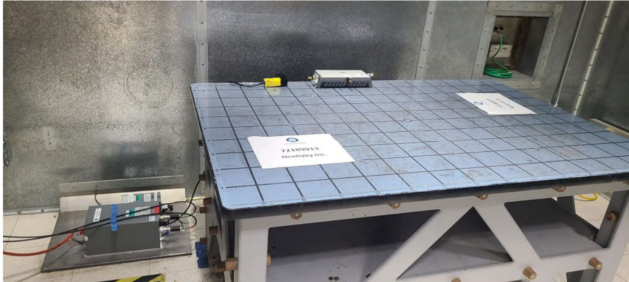
FCC Part 15.247 AC Mains Conducted Emissions Test Setup
