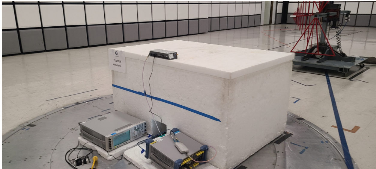
FCC Part 2.1053 Radiated Emissions Test Setup (30 MHz to 1 GHz)
