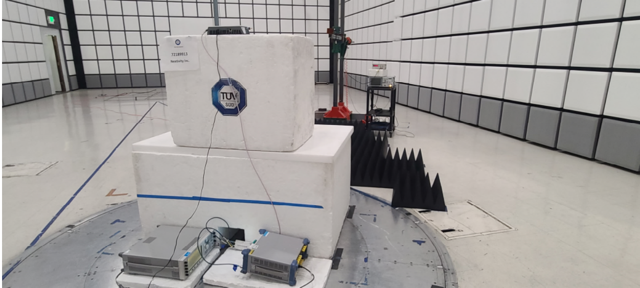
FCC Part 2.1053 Radiated Emissions Test Setup (1 GHz to 26 GHz)
