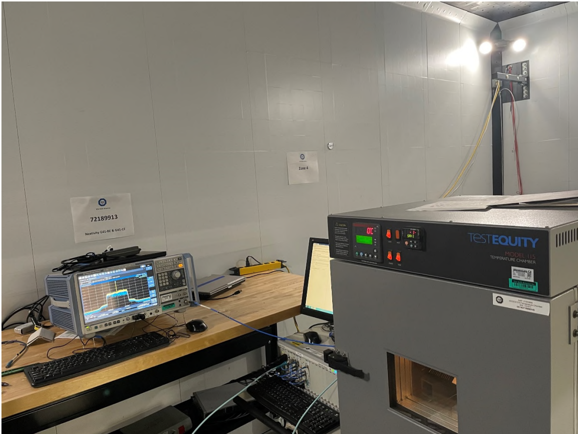
Frequency Stability Test Setup
