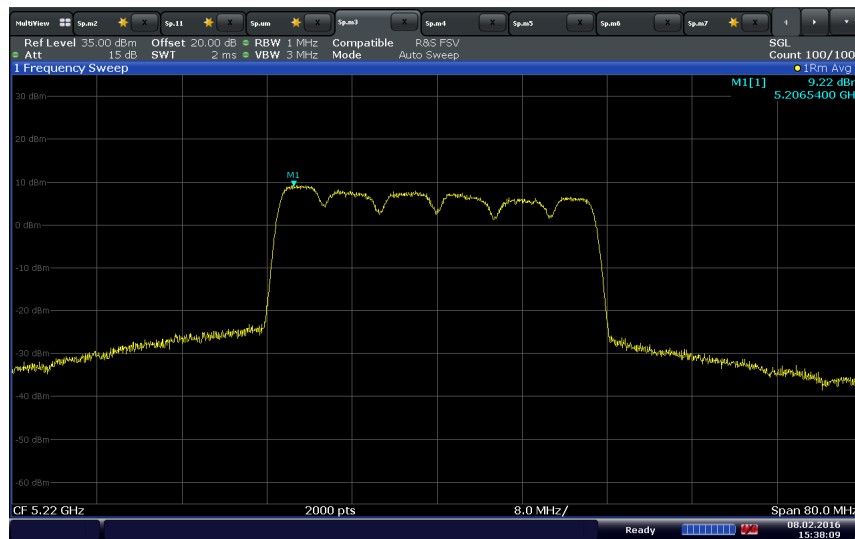
UNII 1 30MHz Bandwidth Middle Channel 5220 MHz
