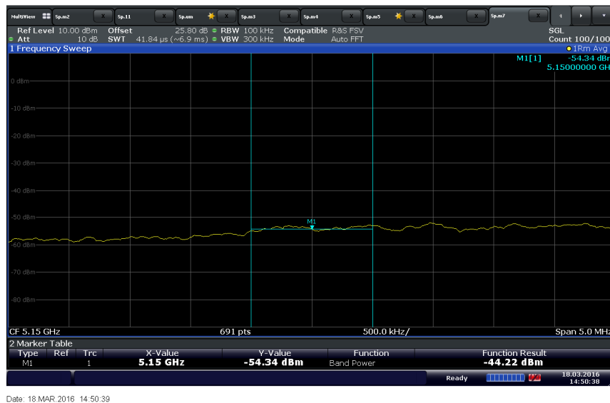
UNII 1 30MHz Lower Band Edge 5150MHz (Average Measurement) @5190MHz
