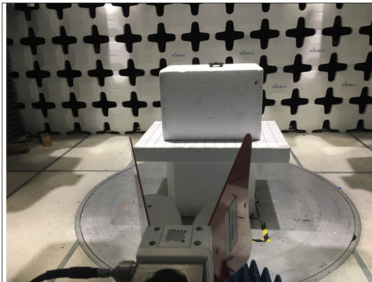
Radiated Emission Test above 1GHz Front View
