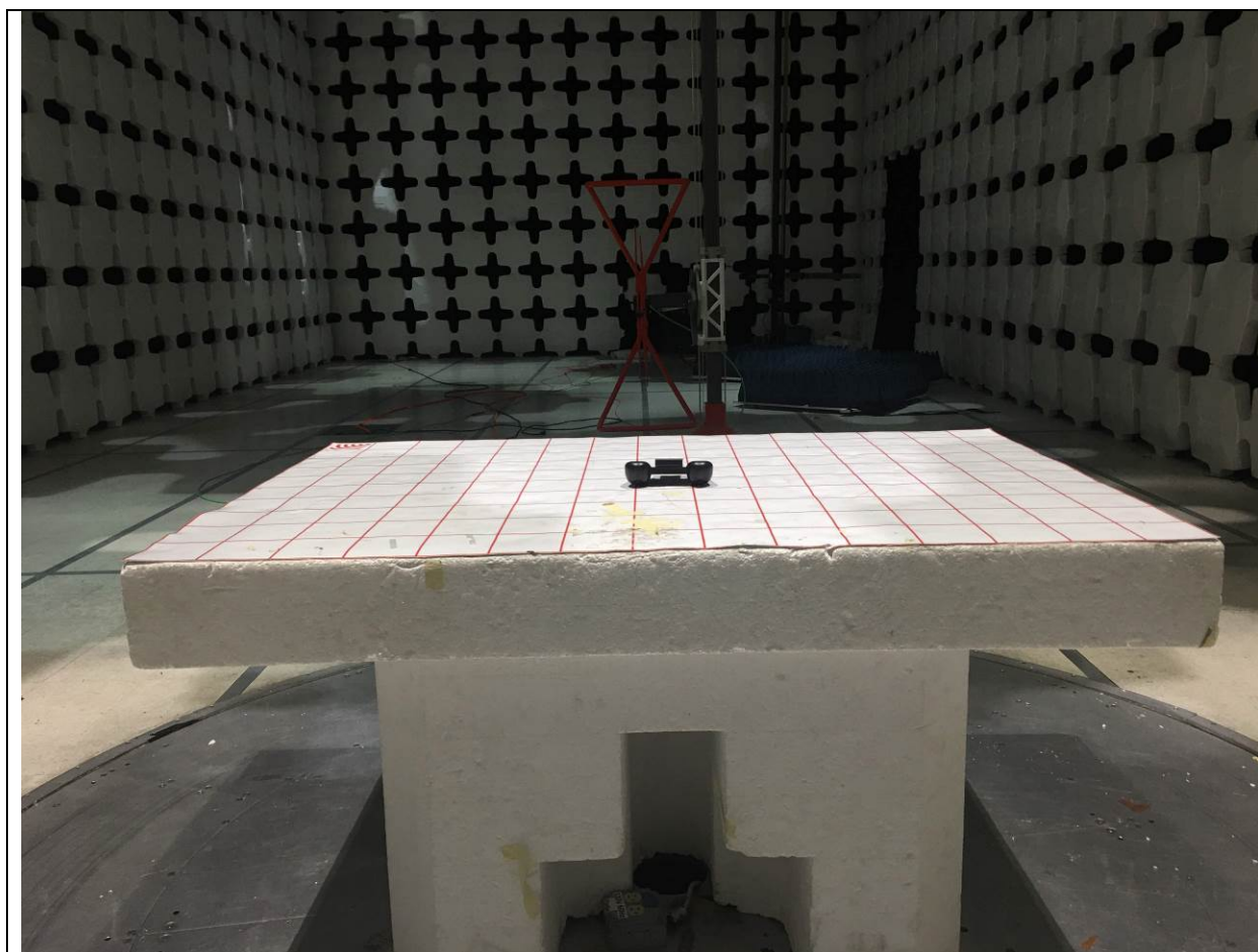
Radiated Emission Test below 1GHz Front View
