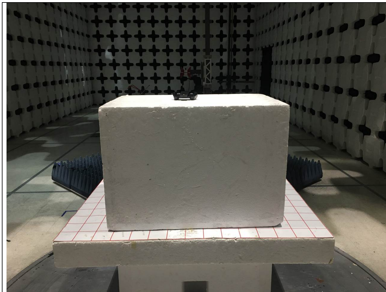
Radiated Emission Test above 1GHz Rear View
