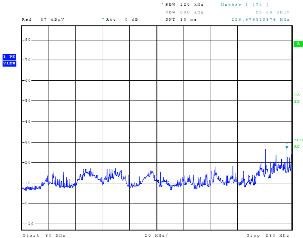
Figure One General Radiated Emissions in screen room
