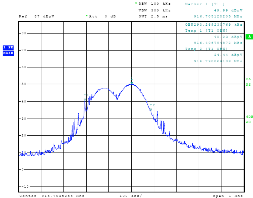
Figure Six Occupied Bandwidth
