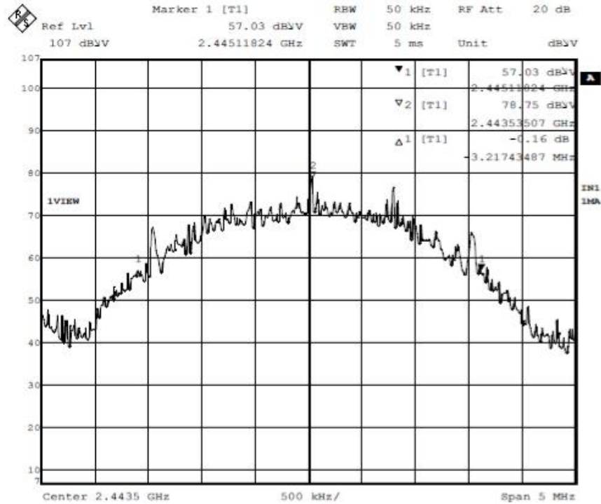
Figure 3 – Result data graph shows 20 dB bandwidth, CF = 2.4435GHz, BW = 3.21MHz
