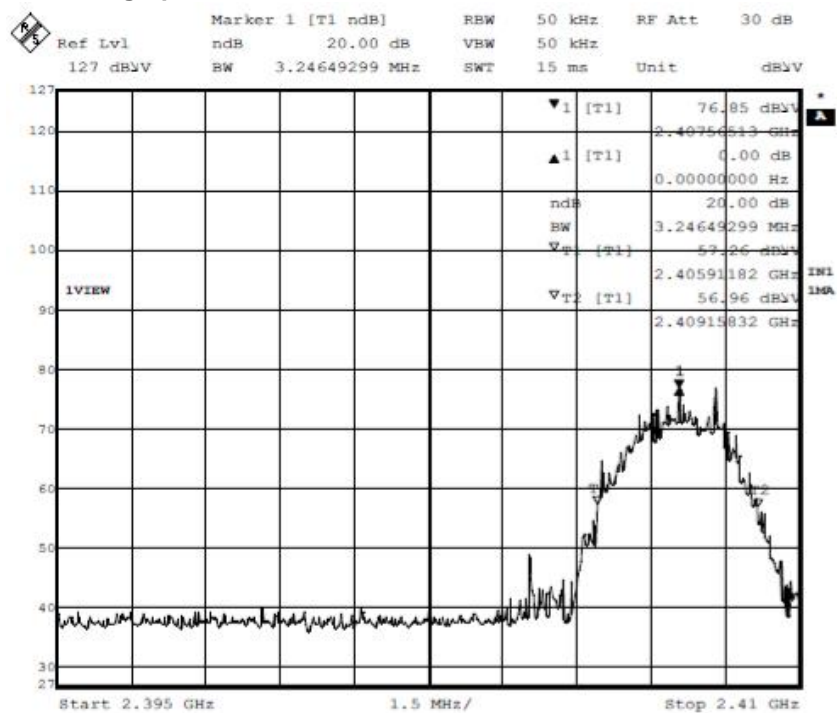
Figure 2 – Result data graph shows 20 dB bandwidth, CF = 2.4075GHz, BW = 3.24MHz
