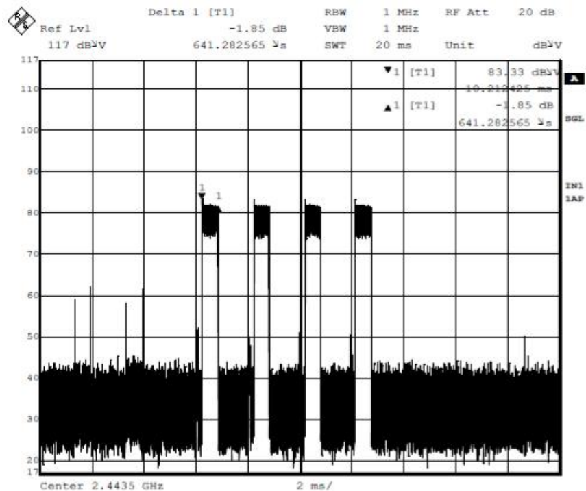
Figure 7 – Result data graph zooms into detail, 4 pulses within 1 set, one pulse period is 641μs.
