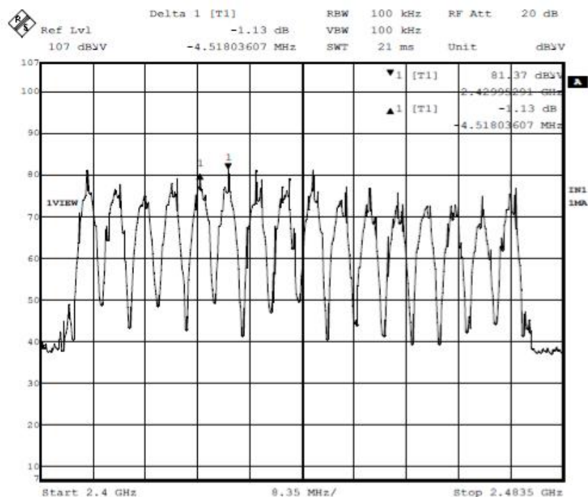
Figure 5 – Result data graph shows the channel separation:
