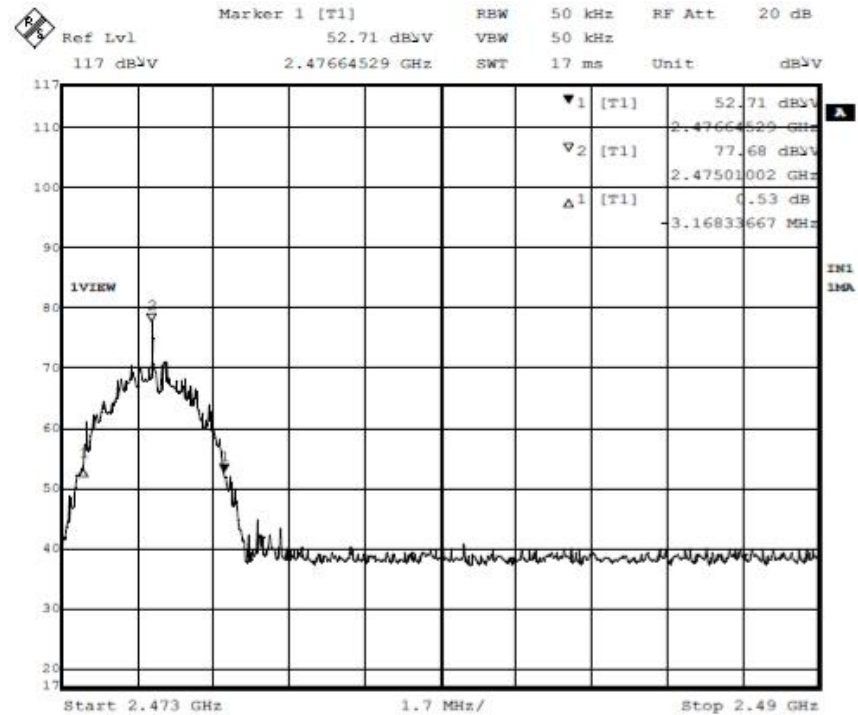
Figure 4 – Result data graph shows 20 dB bandwidth, CF = 2.475GHz, BW = 3.16MHz
