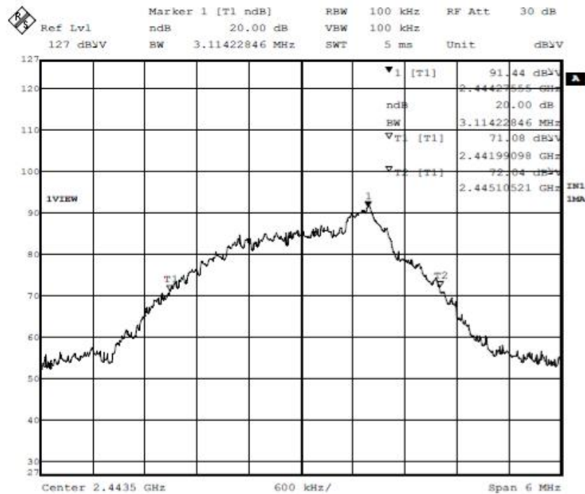
Figure 3 – Result data graph shows 20 dB bandwidth, CF = 2.4435GHz, BW = 3.11MHz
