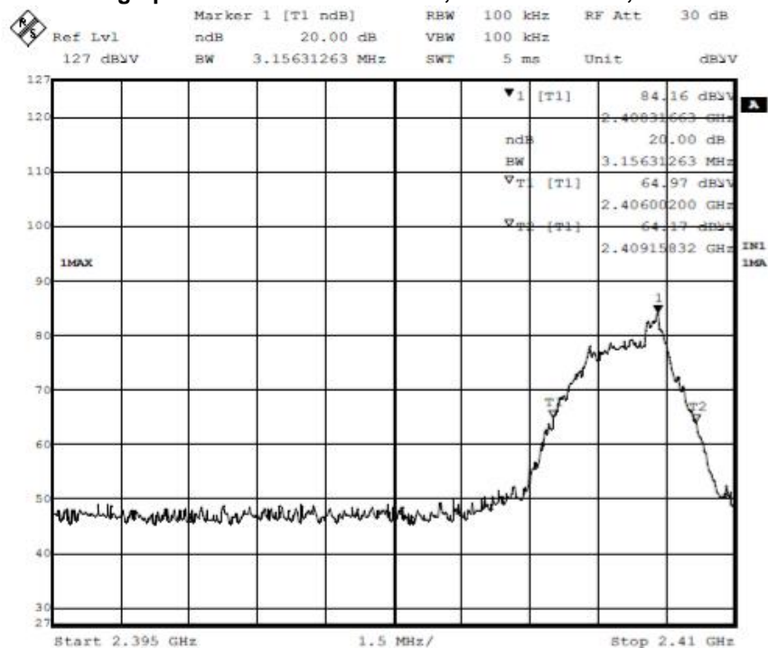
Figure 2 – Result data graph shows 20 dB bandwidth, CF = 2.4075GHz, BW = 3.15MHz
