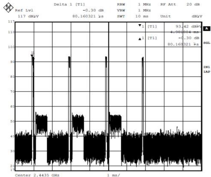
Figure 7 – Result data graph zooms into detail, 4 pulses within 1 set, one pulse period is 80.1μs.
