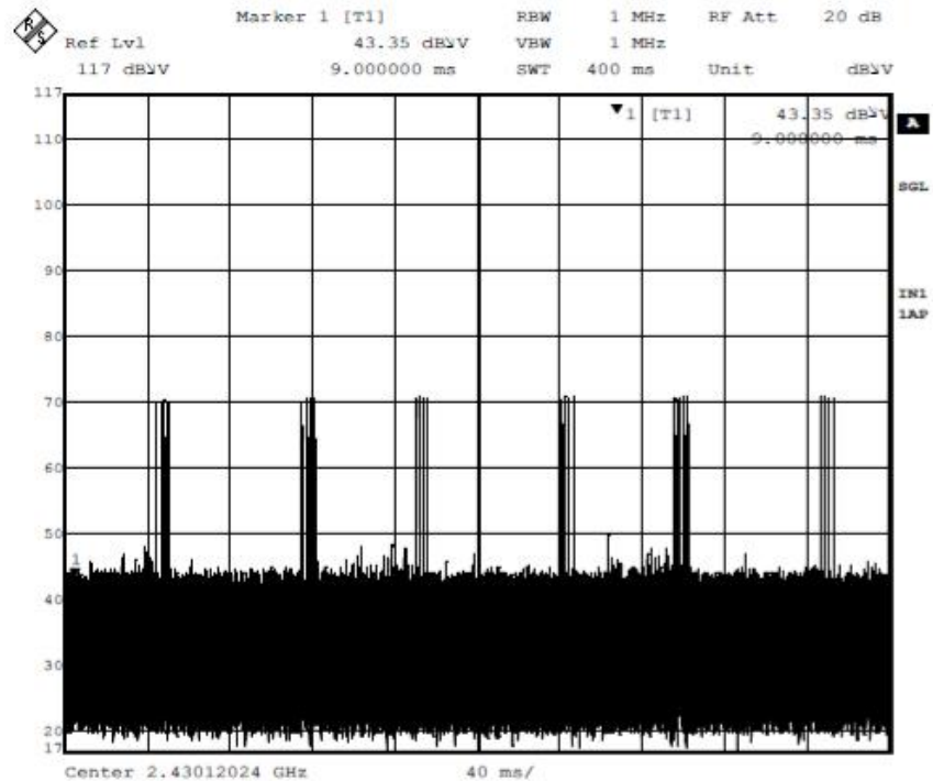
Figure 6 – Result data graph shows total 6 sets of pulses with 400ms.
