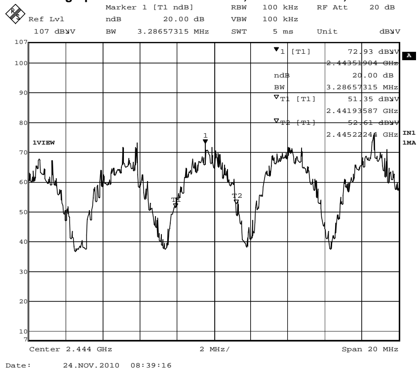
Figure 3 – Result data graph shows 20 dB bandwidth, CF = 2.4435GHz, BW = 3.28MHz
