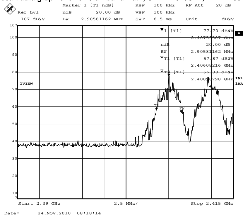
Figure 2 – Result data graph shows 20 dB bandwidth, CF = 2.4075GHz, BW = 2.90MHz
