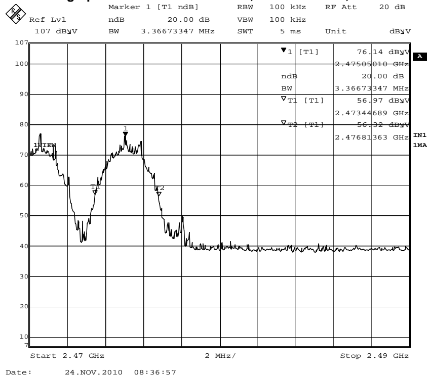
Figure 4 – Result data graph shows 20 dB bandwidth, CF = 2.475GHz, BW = 3.37MHz
