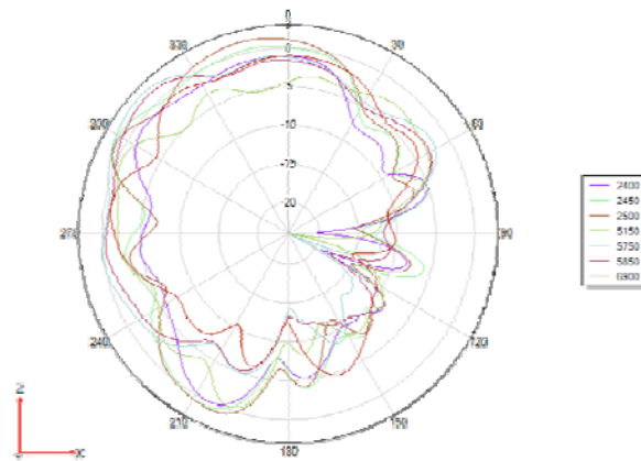
Phi 0°
