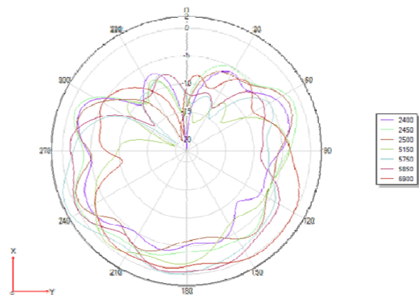
Theta 90°
