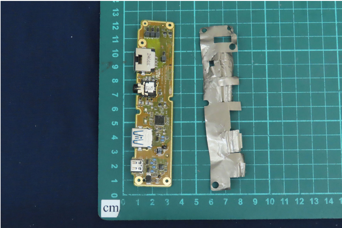
(42) EUT Photo
