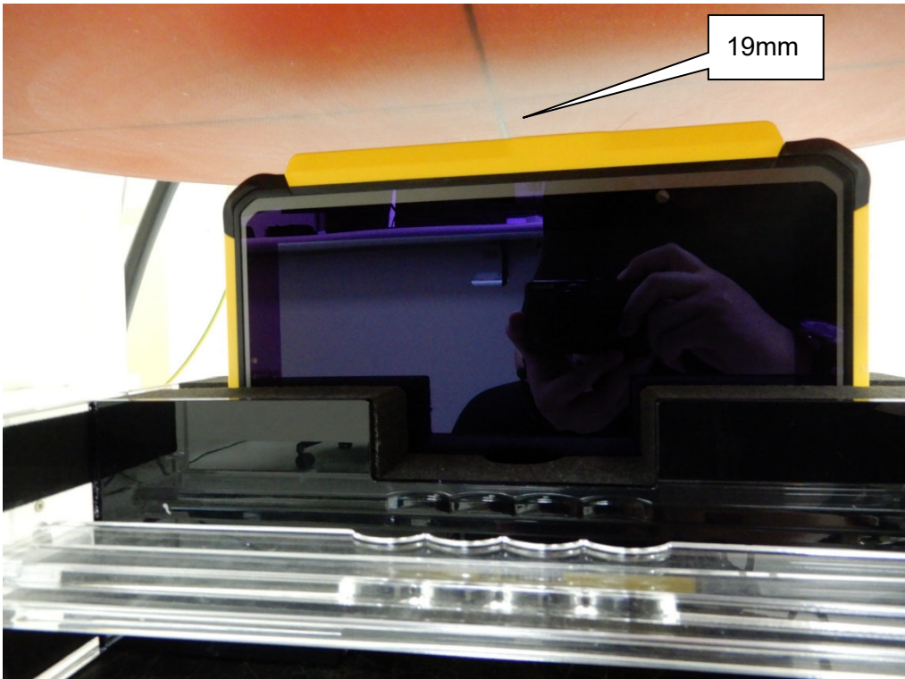
EUT Top_19mm
