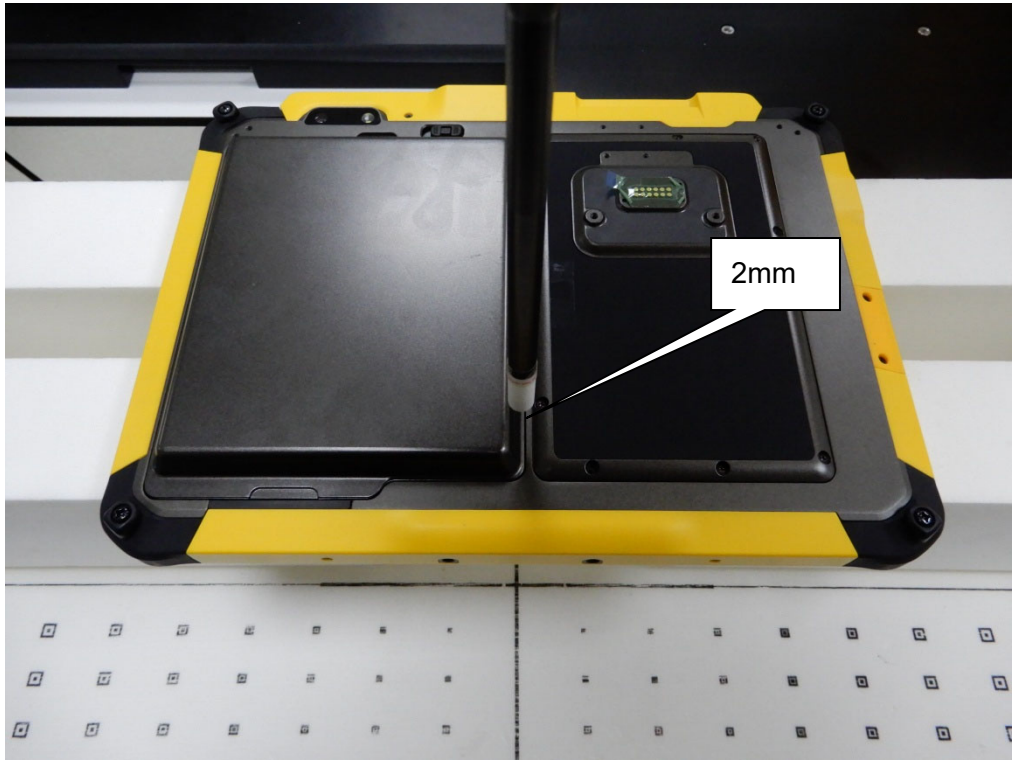
EUT Back_PD_2mm
