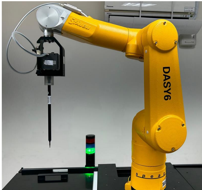
Fig.1 Photograph of the SAR measurement system
