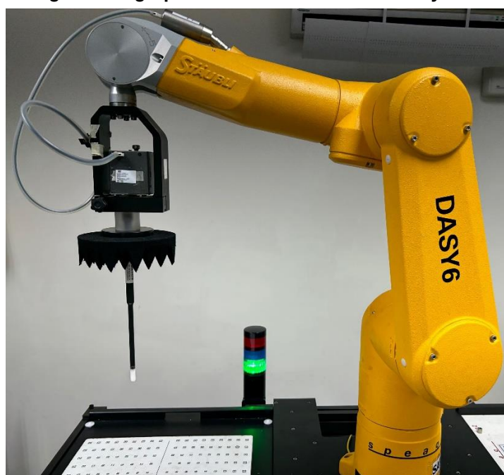
Fig.2 Photograph of the mmW measurement system
